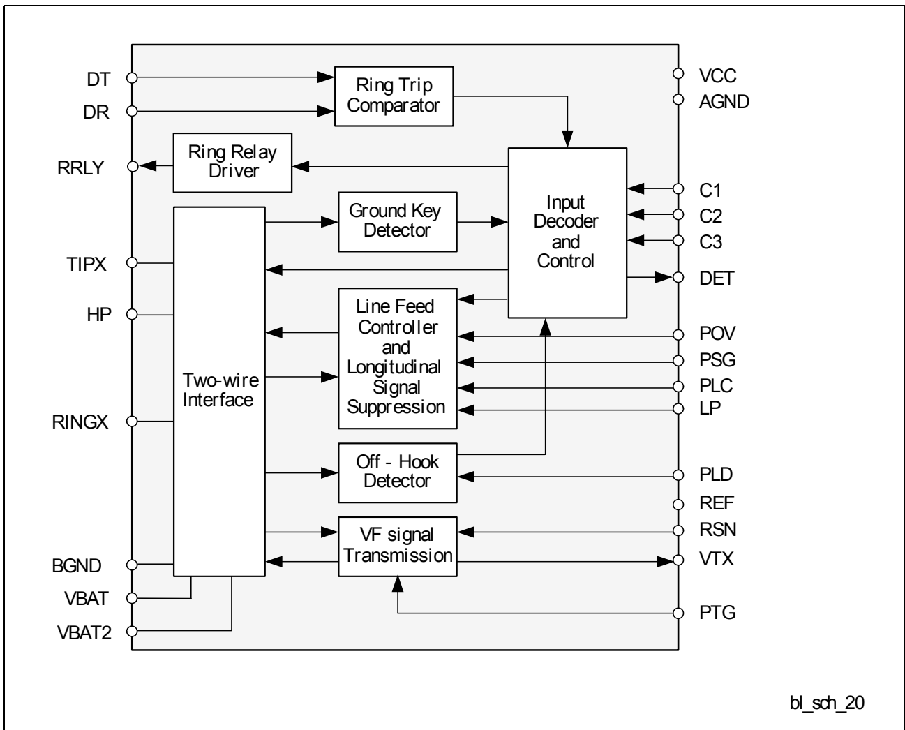
Figure 1 Block Diagram
