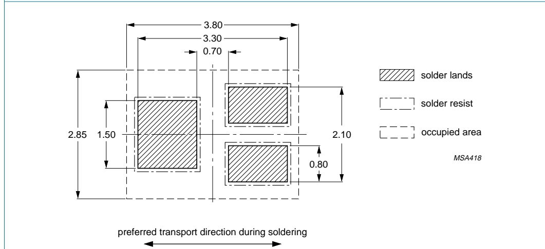
Fig 12. Reflow soldering footprint
