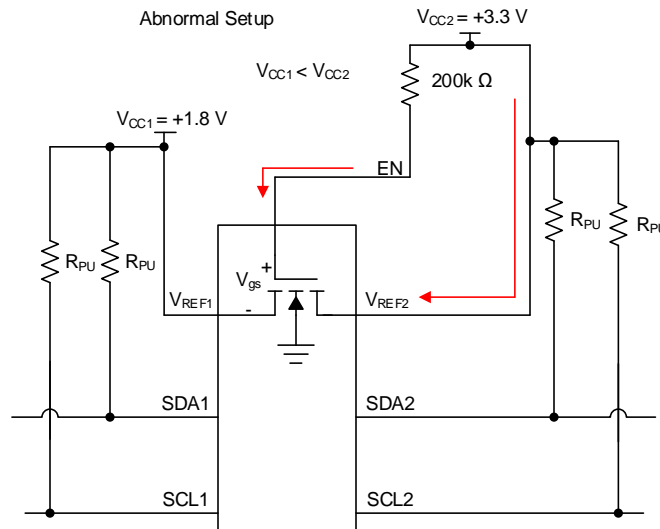
Figure 7. Abnormal Setup
