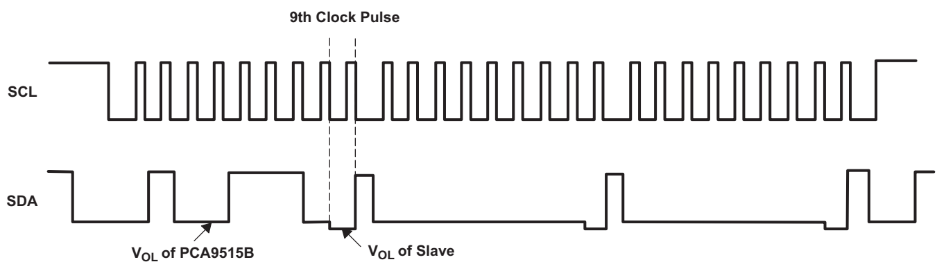
Figure 7. Bus 1 Waveforms
