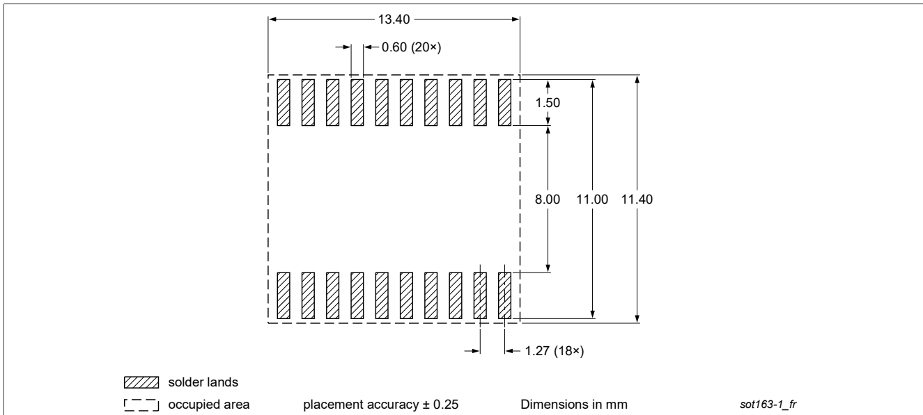
Figure 24. PCB footprint for SOT163-1 (SO20); reflow soldering
