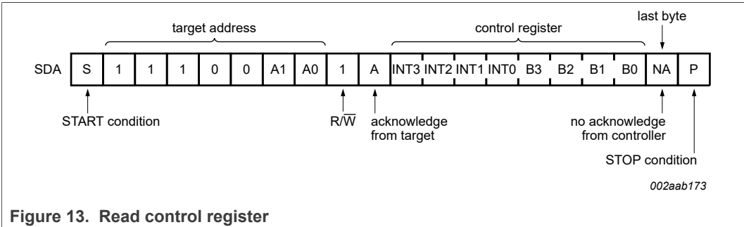
Figure 13. Read control register
