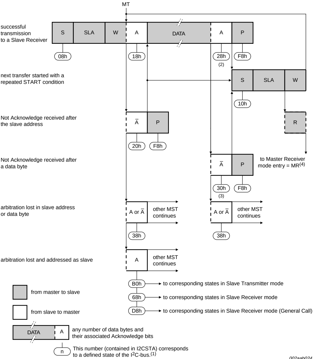
(1) See Table 27 (2) Defined state when a single byte is sent and an ACK is received. (3) Defined state when a single byte is sent and a NACK is received. (4) Master Receiver Byte mode is entered when MODE = 0. Master Receiver Buffered mode is entered when MODE = 1. Fig 7. Format and states in the Master Transmitter Byte mode (MODE = 0)
