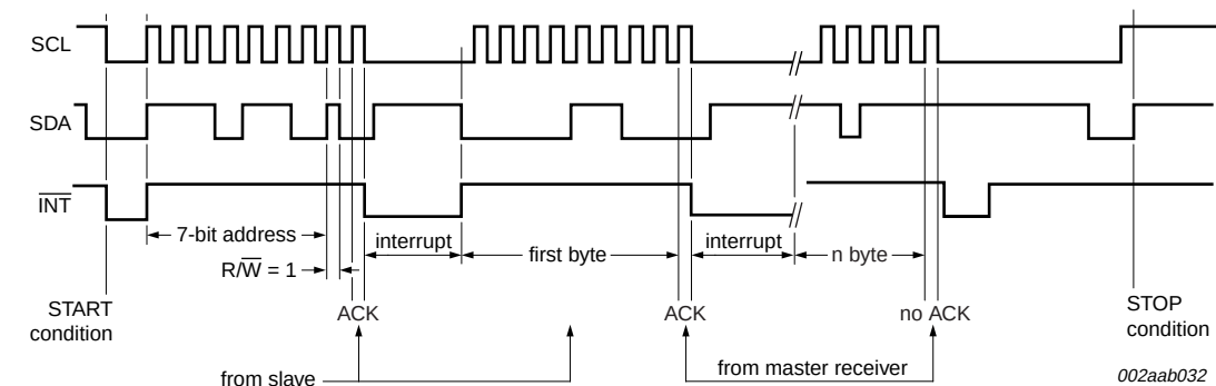
Fig 21. Bus timing diagram; Unbuffered Master Receiver mode
