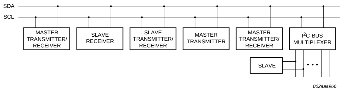
Fig 30. System configuration
