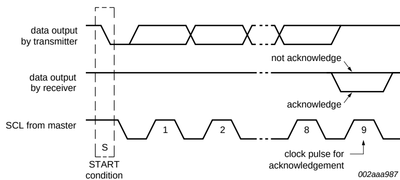
Fig 31. Acknowledgement on the I 2 C-bus
