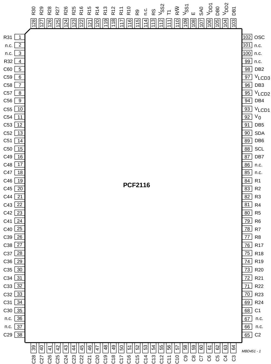
Fig.2 Pin configuration (LQFP128).
