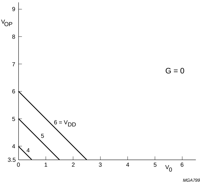
b. Buffer mode V_{OP} = V_{DD} - V_0 .
