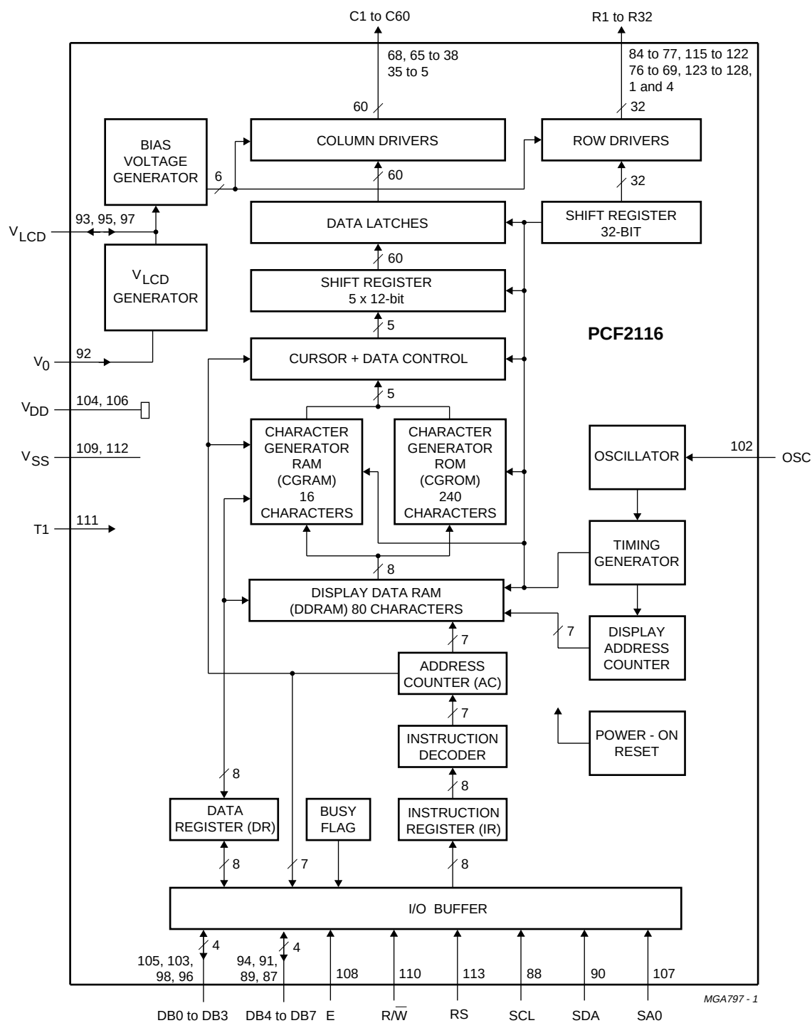
Fig.1 Block diagram (pin numbers for LQFP128 package).
