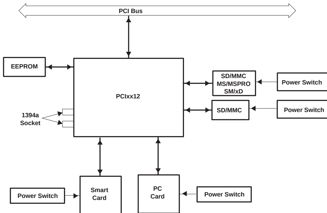
Figure 3–1. PClxx12 System Block Diagram
