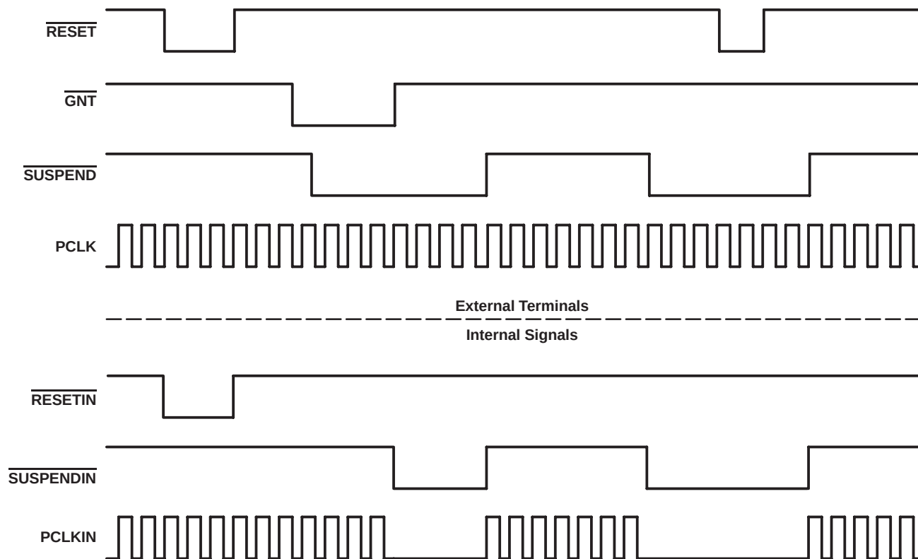
Figure 3–14. Signal Diagram of Suspend Function
