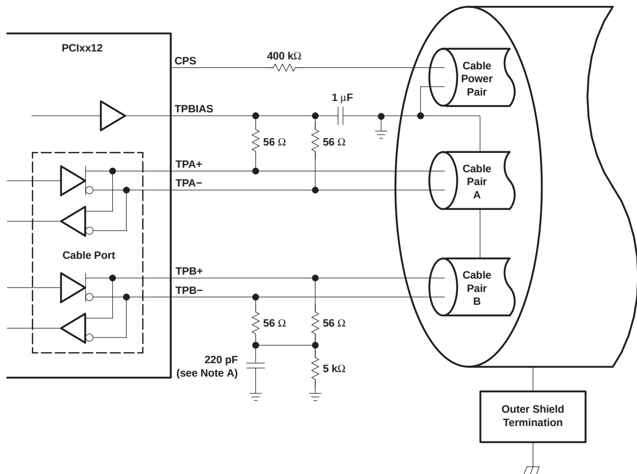
Figure 3-17. TP Cable Connections
