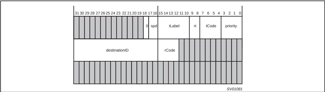
Figure 15. Quadlet/Block Write Response Transmit Format
