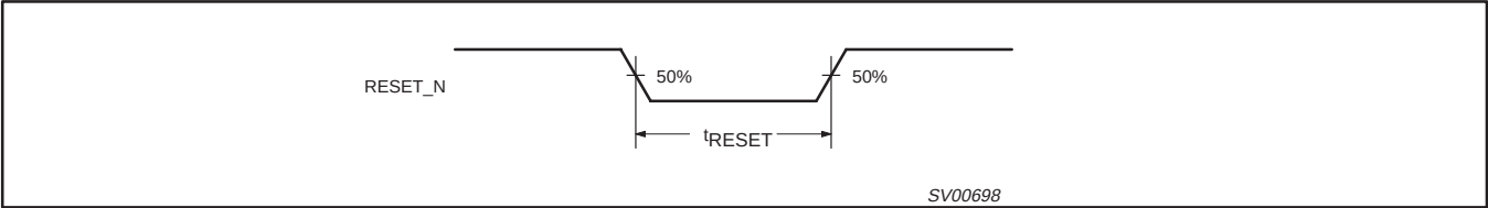
Figure 43. RESET_N Waveform
