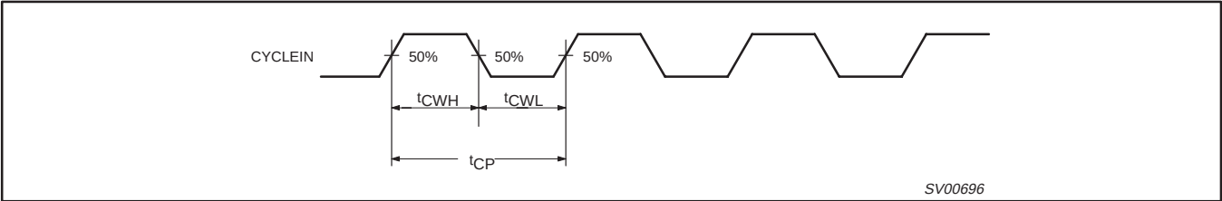
Figure 41. CYCLEIN Waveform
