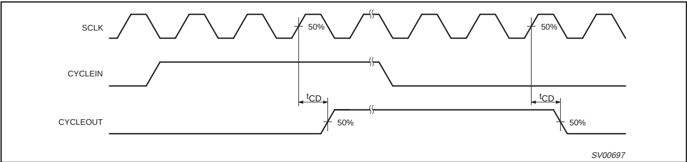
Figure 42. CYCLEOUT Waveforms
