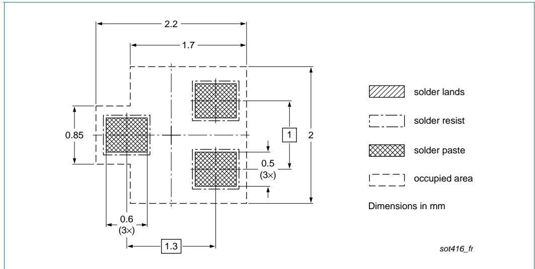
Fig 16. Reflow soldering footprint PDTC114YE (SOT416/SC-75)
