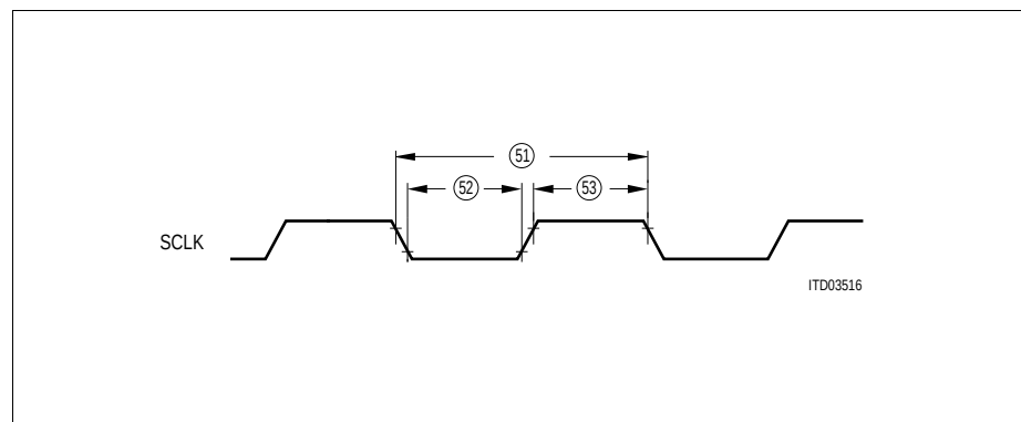
Figure 124 Clock Timing
