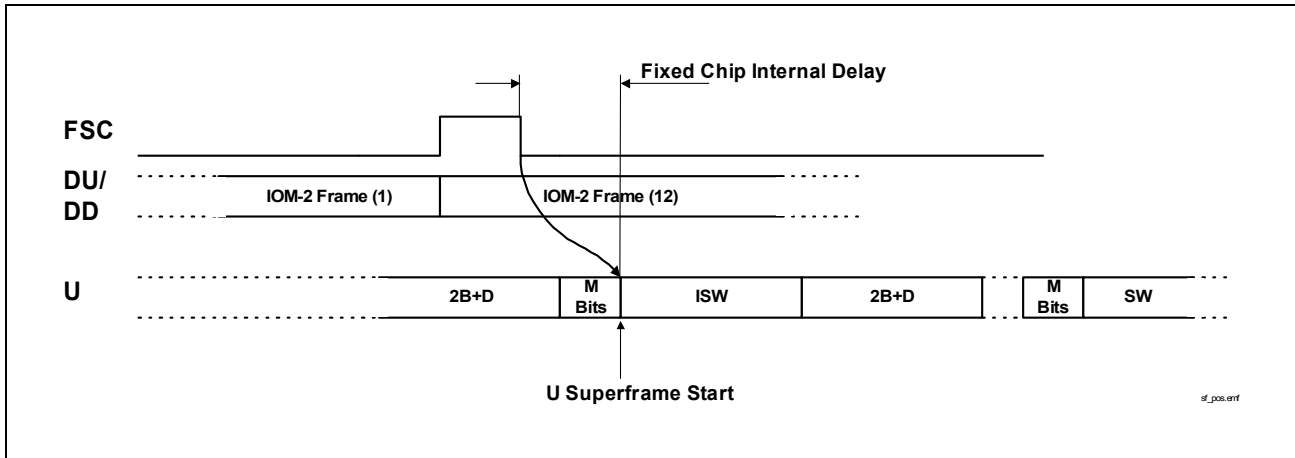
Figure 11 Superframe Marker
