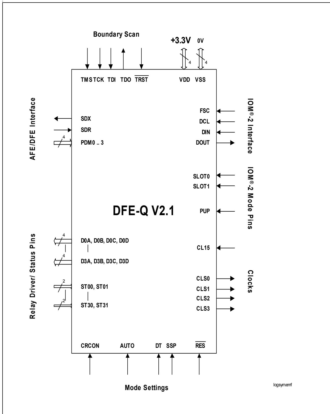
Figure 2 Logic Symbol
