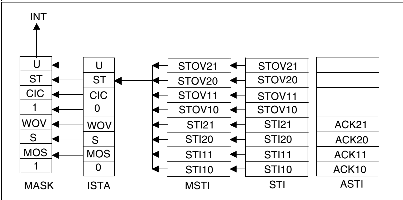
Figure 17 Interrupt Structure of the Synchronous Data Transfer
