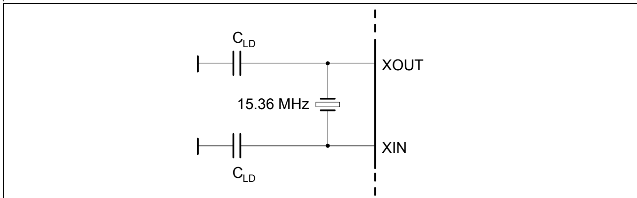
Figure 57 Crystal Oscillator
