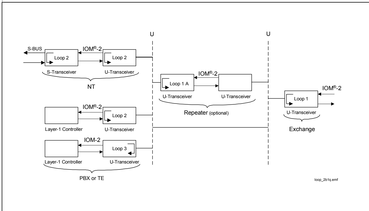
Figure 49 Test Loopbacks
