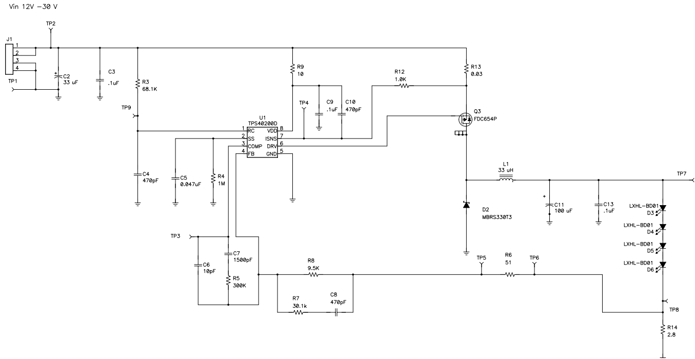
Figure 44. Wide-Input-Voltage Range LED Driver
