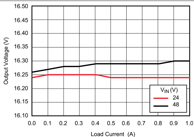
Figure 43. Load Regulation, Two Input Voltage Extremes
