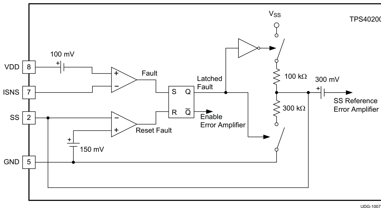
Figure 26. Current-Limit Reset
