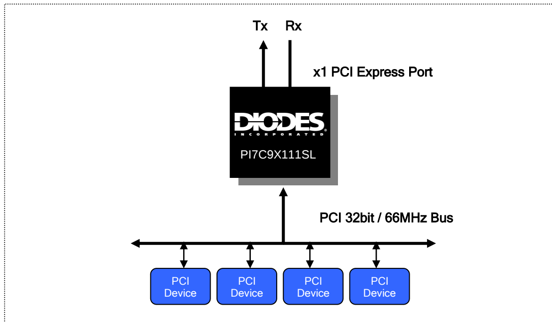
Figure 1-1 PI7C9X111SL Topology
