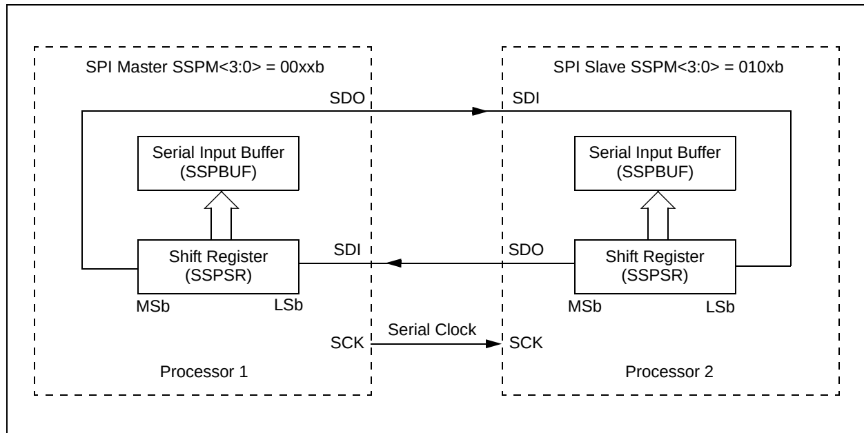
FIGURE 13-2: SPI MASTER/S�AVE CONNECTION
