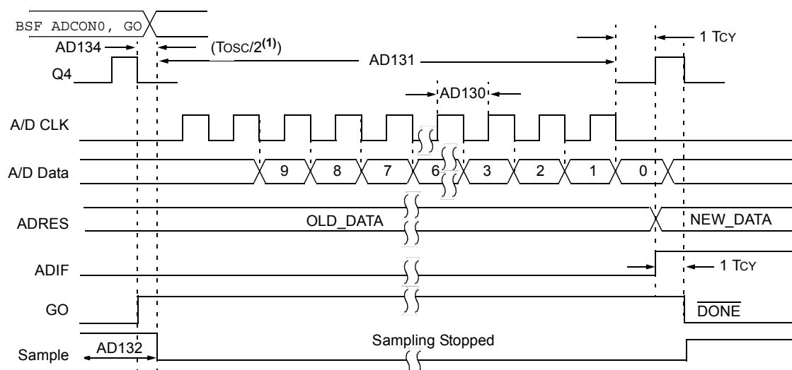
FIGURE 19-9: PIC16F913/914/916/917/946 A/D CONVERSION TIMING (NORMAL MODE)
