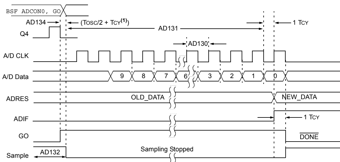
FIGURE 19-10: PIC16F913/914/916/917/946 A/D CONVERSION TIMING (SLEEP MODE)
