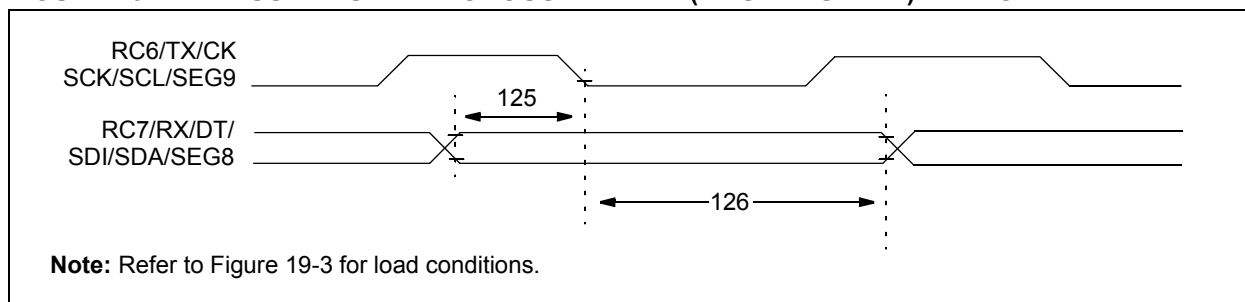
FIGURE 19-12: USART SYNCHRONOUS RECEIVE (MASTER/SLAVE) TIMING
