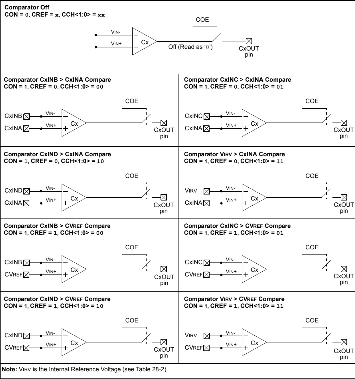
FIGURE 23-4: COMPARATOR CONFIGURATIONS
