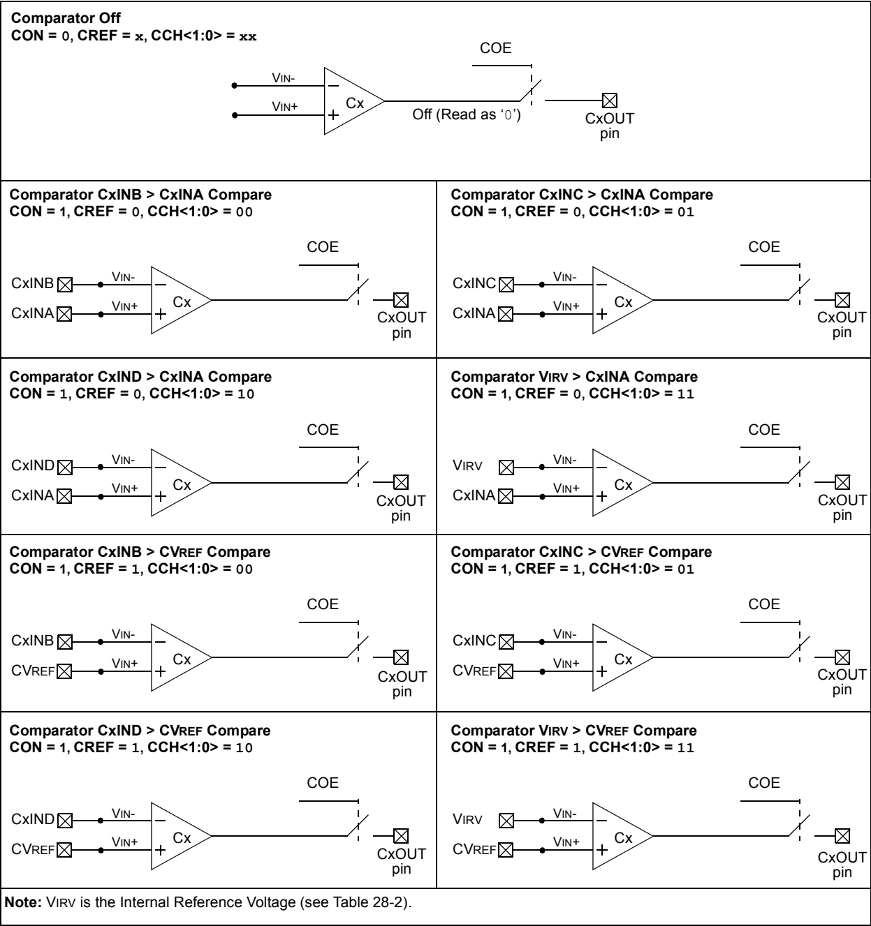
FIGURE 23-4: COMPARATOR CONFIGURATIONS
