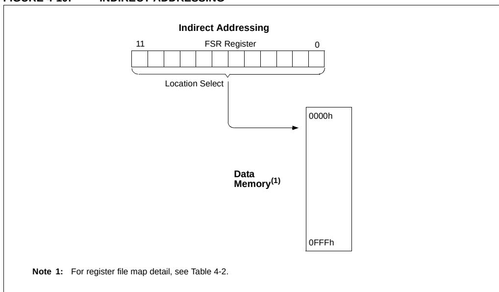
FIGURE 4-10: INDIRECT ADDRESSING
