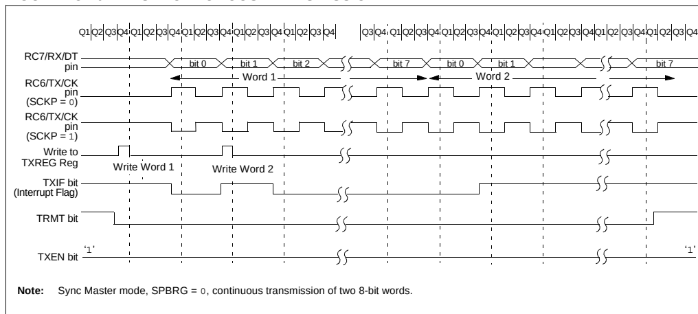
FIGURE 18-10: SYNCHRONOUS TRANSMISSION
