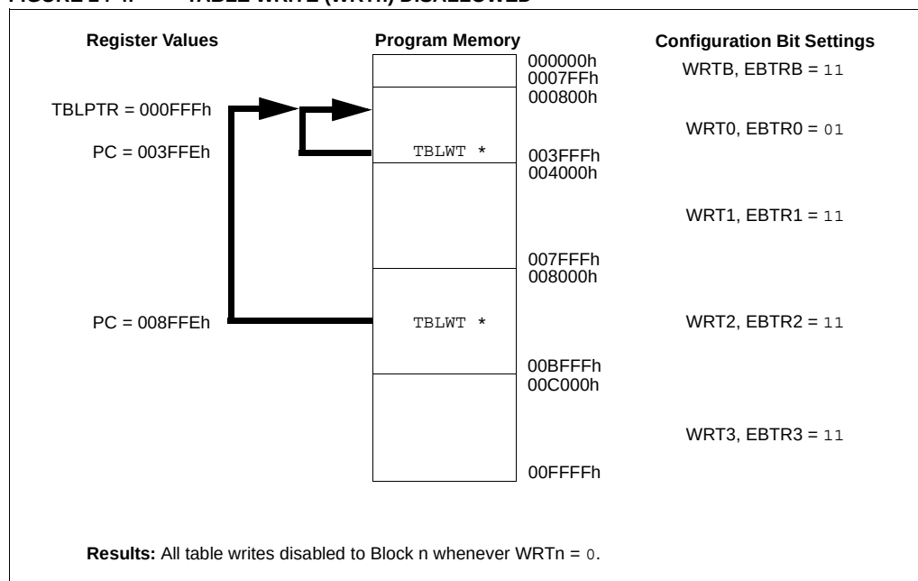
FIGURE 24-4: TABLE WRITE (WRTn) DISABLED
