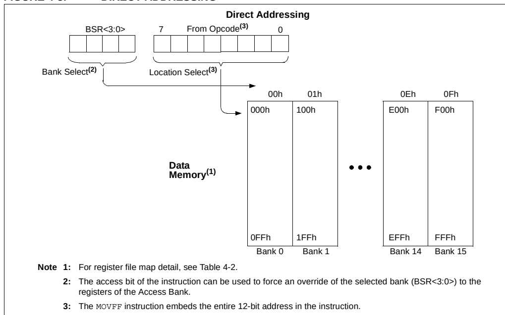
FIGURE 4-8: DIRECT ADDRESSING
