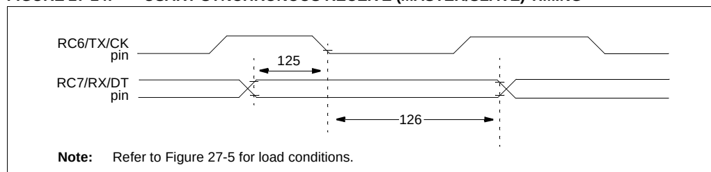
FIGURE 27-24: USART SYNCHRONOUS RECEIVE (MASTER/SLAVE) TIMING
