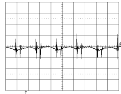
Output voltage ripple (20mV/div.) at: T_{ref} = +25^{\circ}C , I_O = 26 A resistive load, V_i = 12.0 V. Time scale: 1 μs/div. See the filter in the Output ripple and noise section (EMC Specification).
