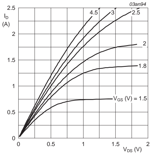
T_j = 25^\circ\text{C}
