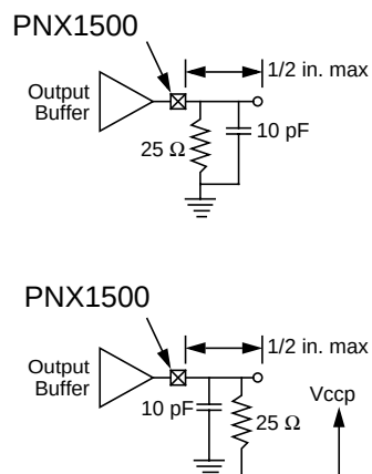
Figure 11: PCI T_{val(max)} Rising and Falling Edge
