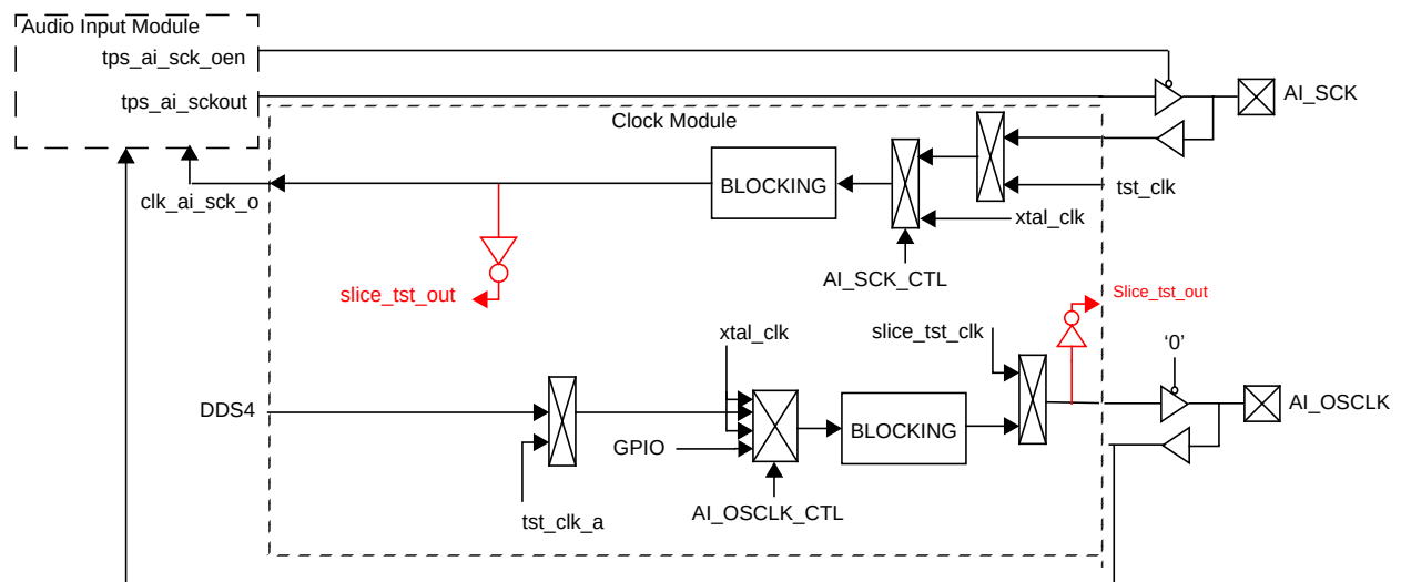
Figure 20: AI Clocks
