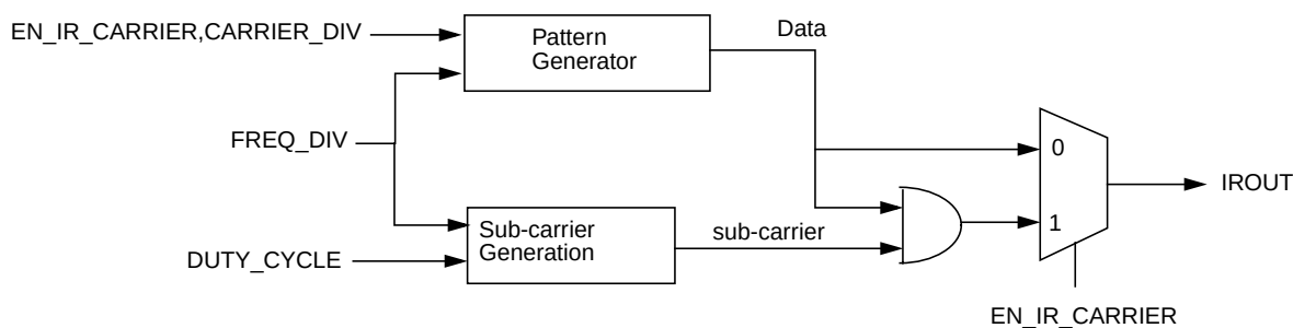
Figure 10: Sub-Carrier Multiplexing for TX
