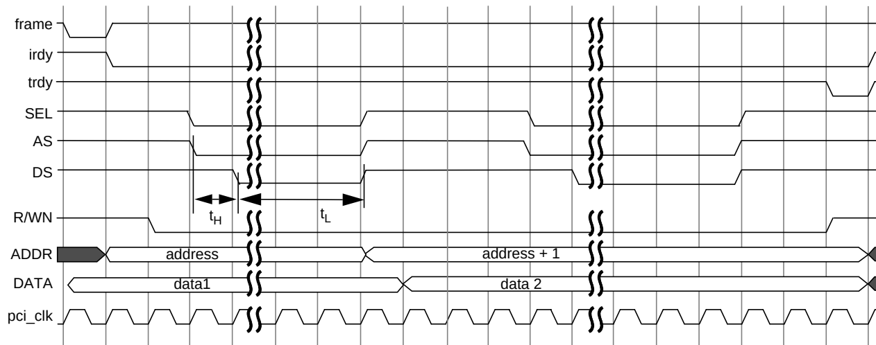
Figure 7: Motorola Write Without DSACK
