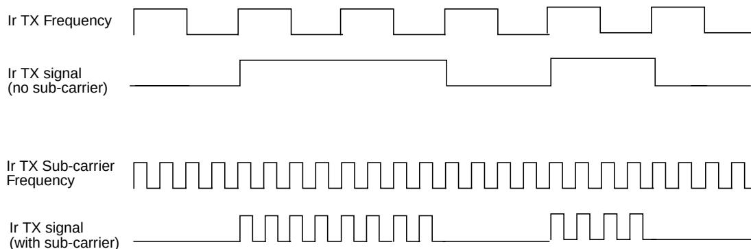
Figure 8: Example of Ir TX Signals with and without Sub-Carrier
