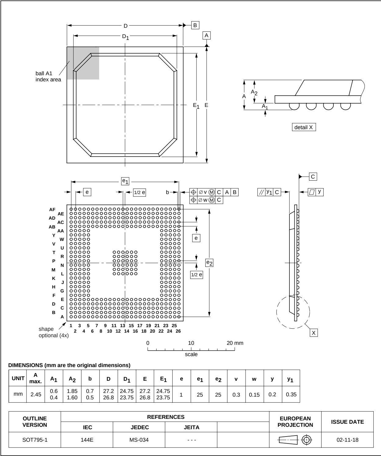
Figure 23: BGA456 Plastic Ball grid Array; 456 Balls; body 27 x 27 x 1.75 mm
