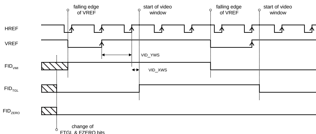
Figure 10: Field Identifier Timing
