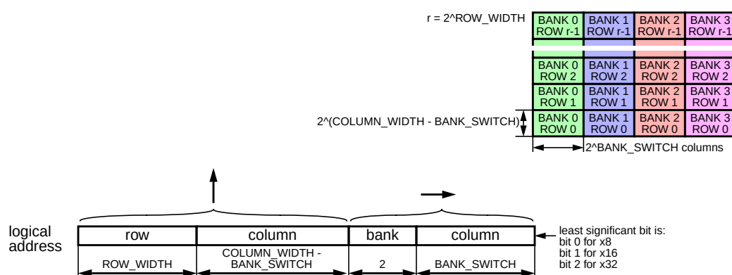
Figure 6: Address Mapping: Interleaved Mode
