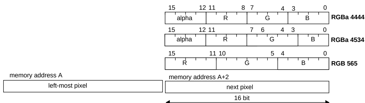
Figure 3: 16-Bit Pixel-Packed Formats
