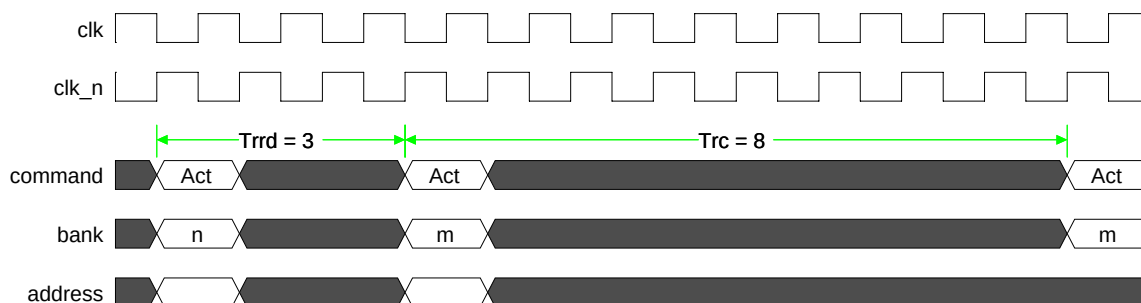
Figure 10: Trrd and Trc Timing Parameters
