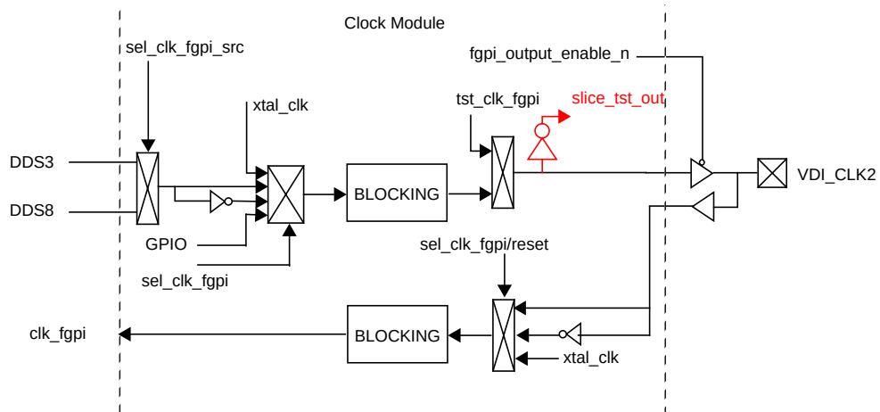
Figure 16: VDI_CLK2 Block Diagram
