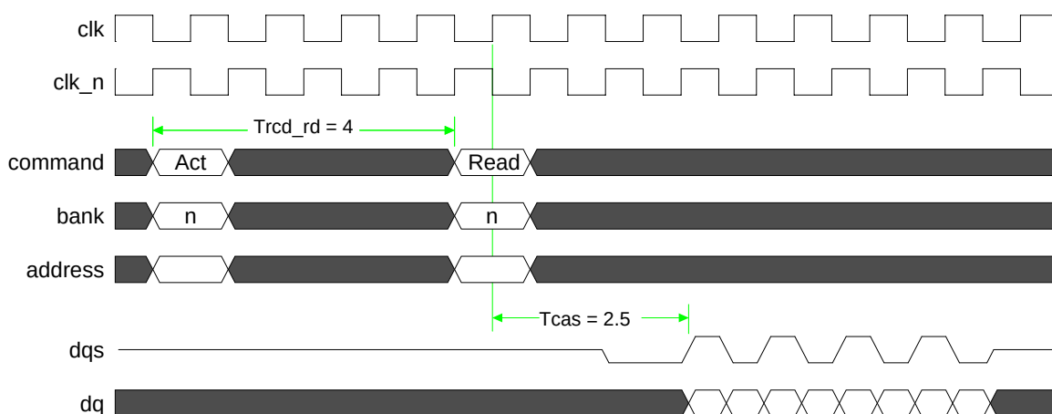
Figure 15: Trcd_rd Timing Parameter
