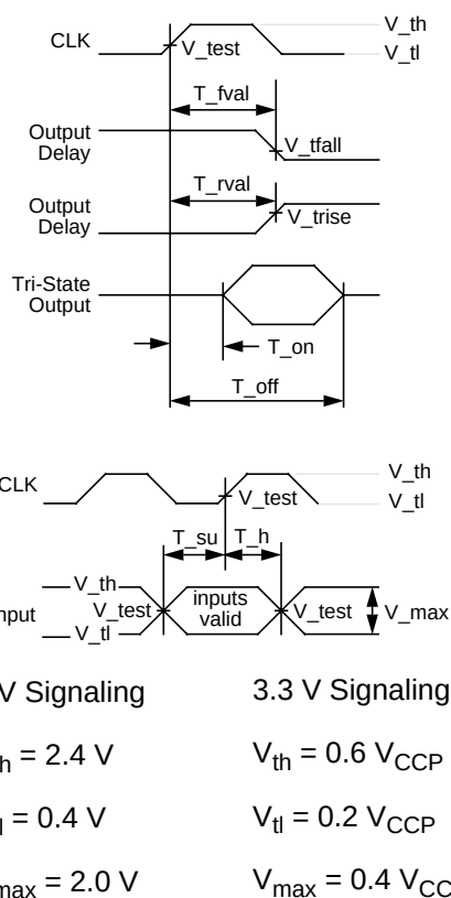
Figure 10: PCI Output and Input Timing Measurement Conditions
