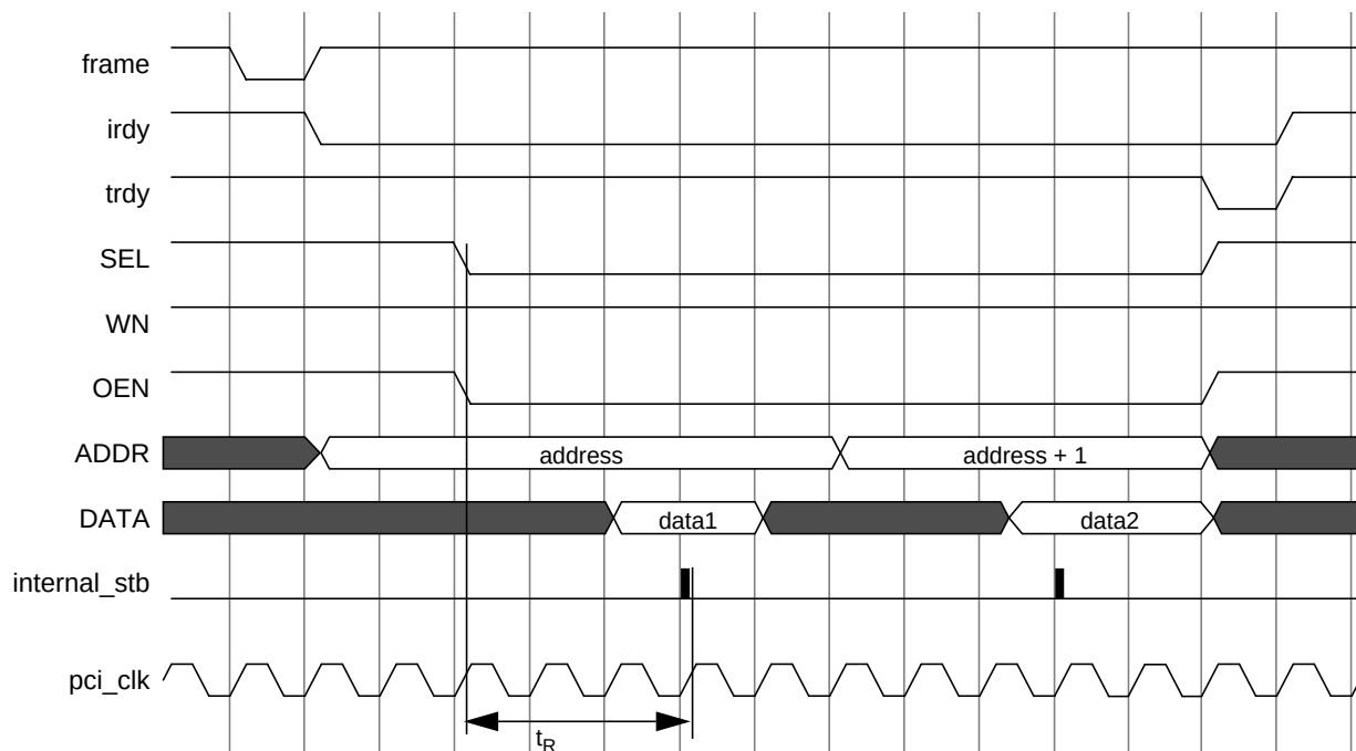
Figure 10: NOR Flash Read
