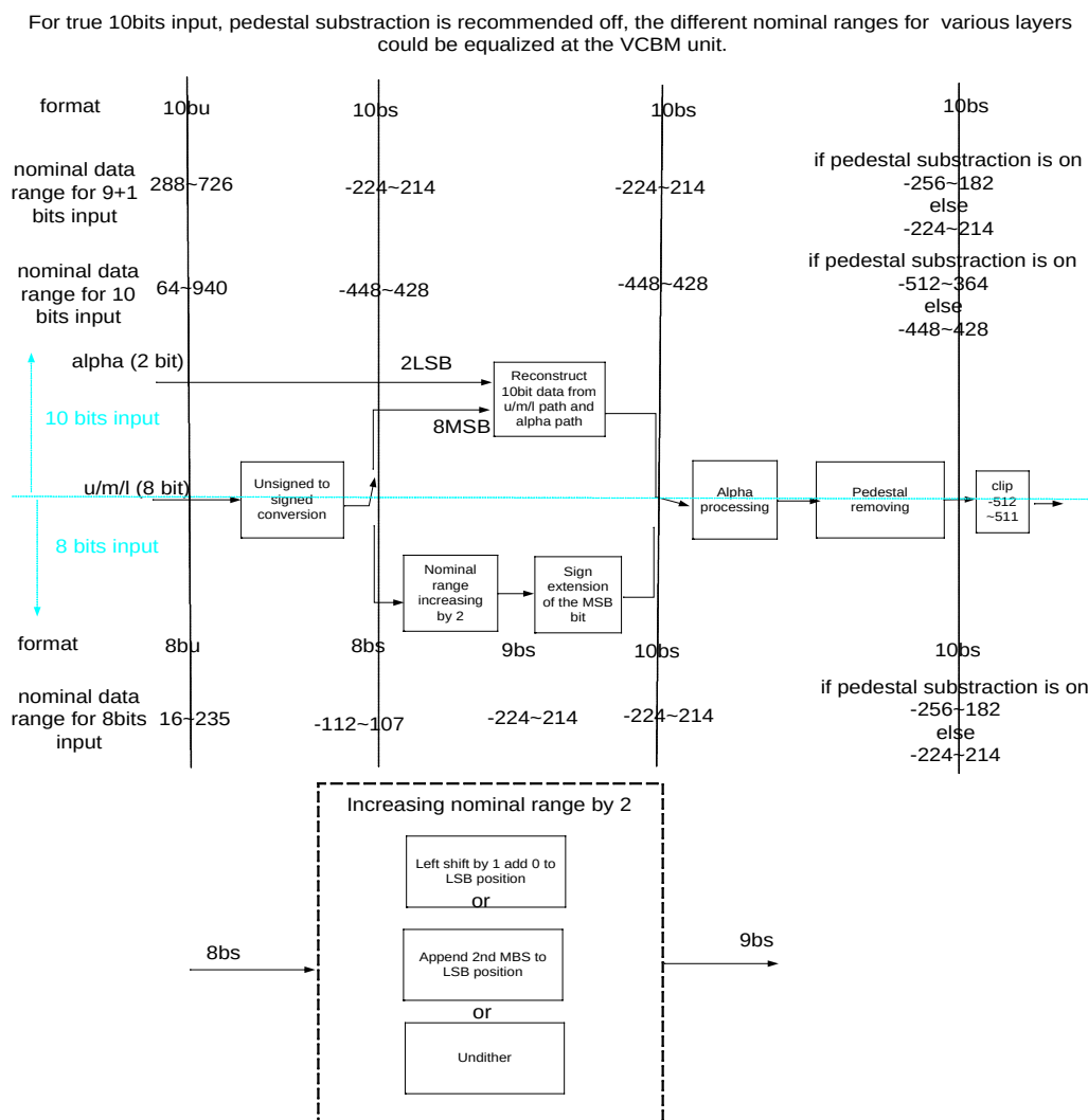
Figure 3: Undithering and Pedestal Manipulation
