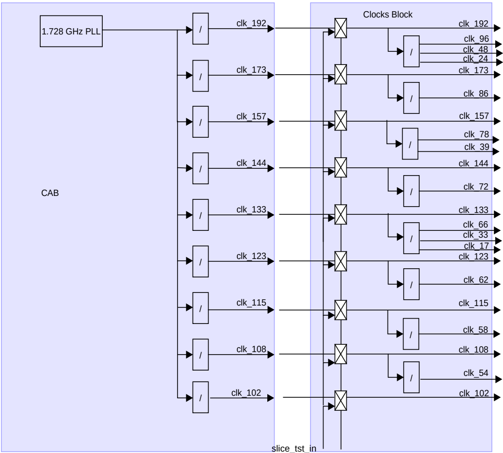
Figure 10: Clock Dividers
