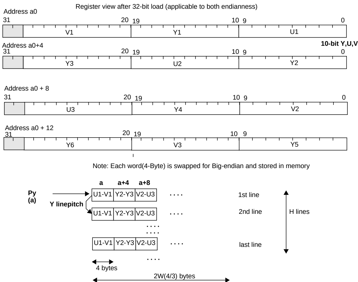
Figure 12: Packed 10-bit YUV 4:2:2 Format
