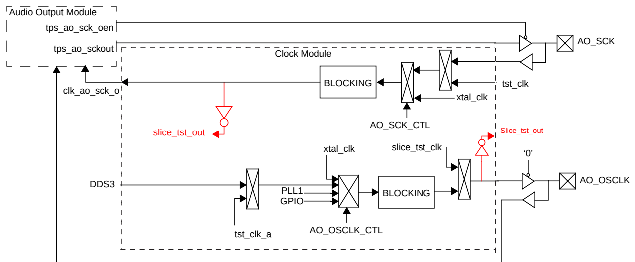
Figure 19: AO Clocks
