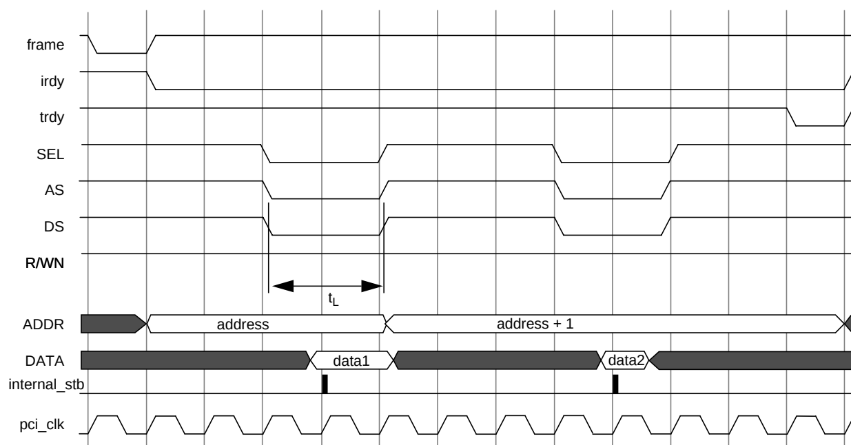
Figure 8: Motorola Read
