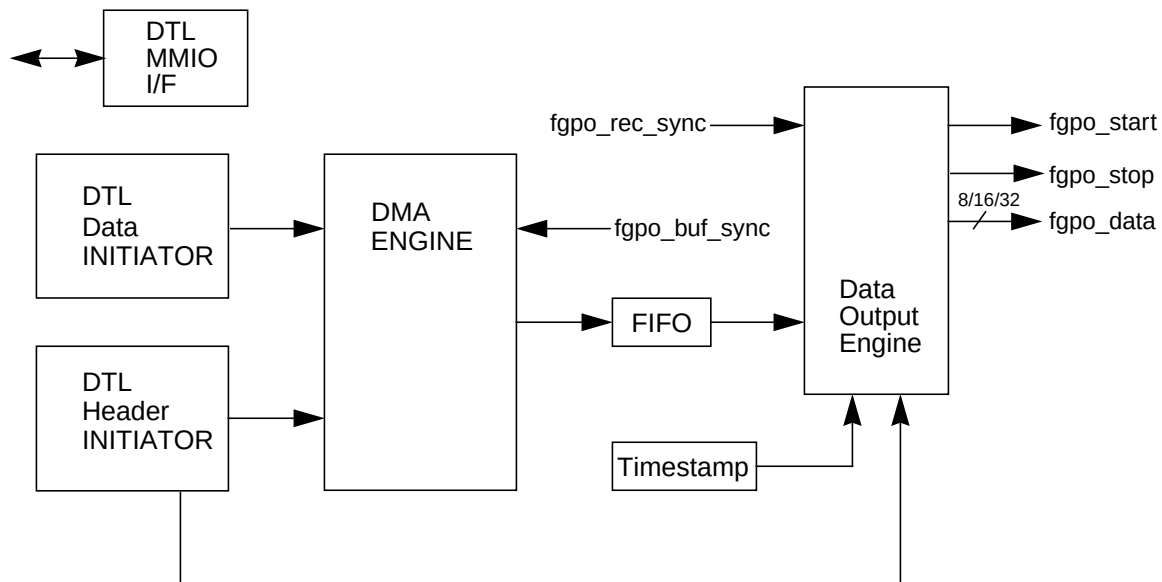
Figure 2: FGPO Module Block Diagram
