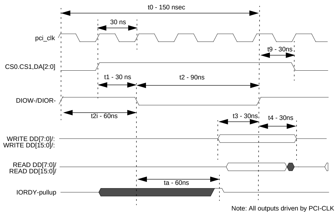
Figure 14: Timings on IDE Bus
