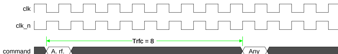
Figure 11: Trfc Timing Parameter
