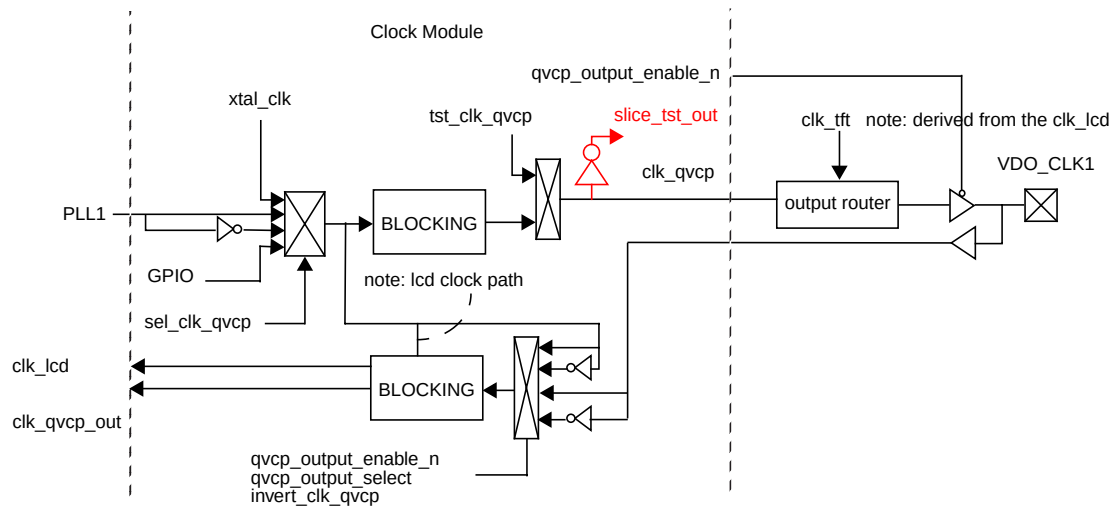
Figure 17: VDO_CLK1 Block Diagram
