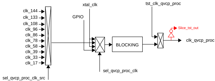
Figure 8: QVCP_PROC Clock
