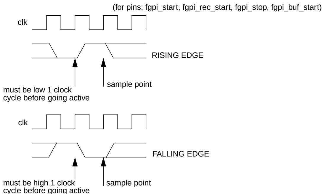
Figure 6: Signal Edge Definition
