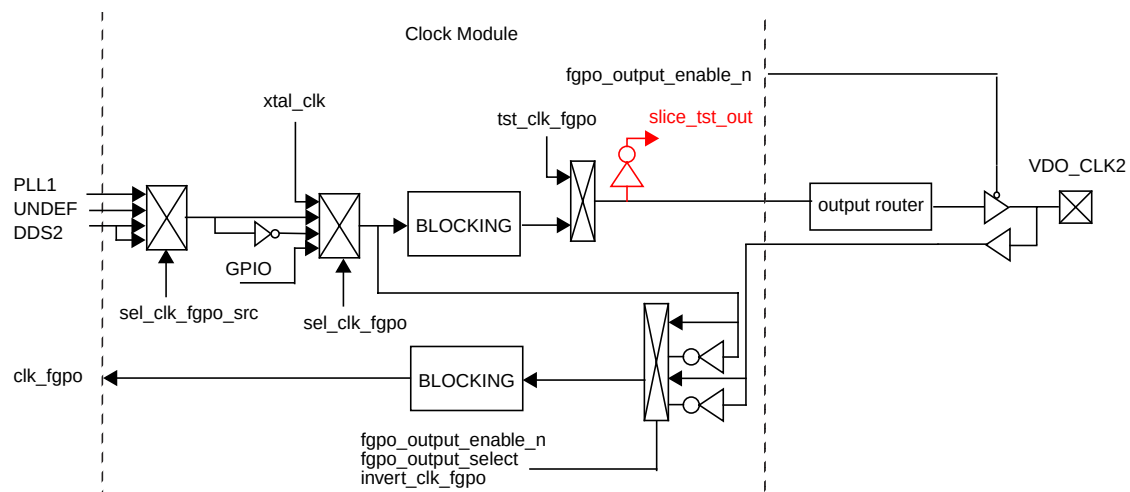
Figure 18: VDO_CLK2 Block Diagram
