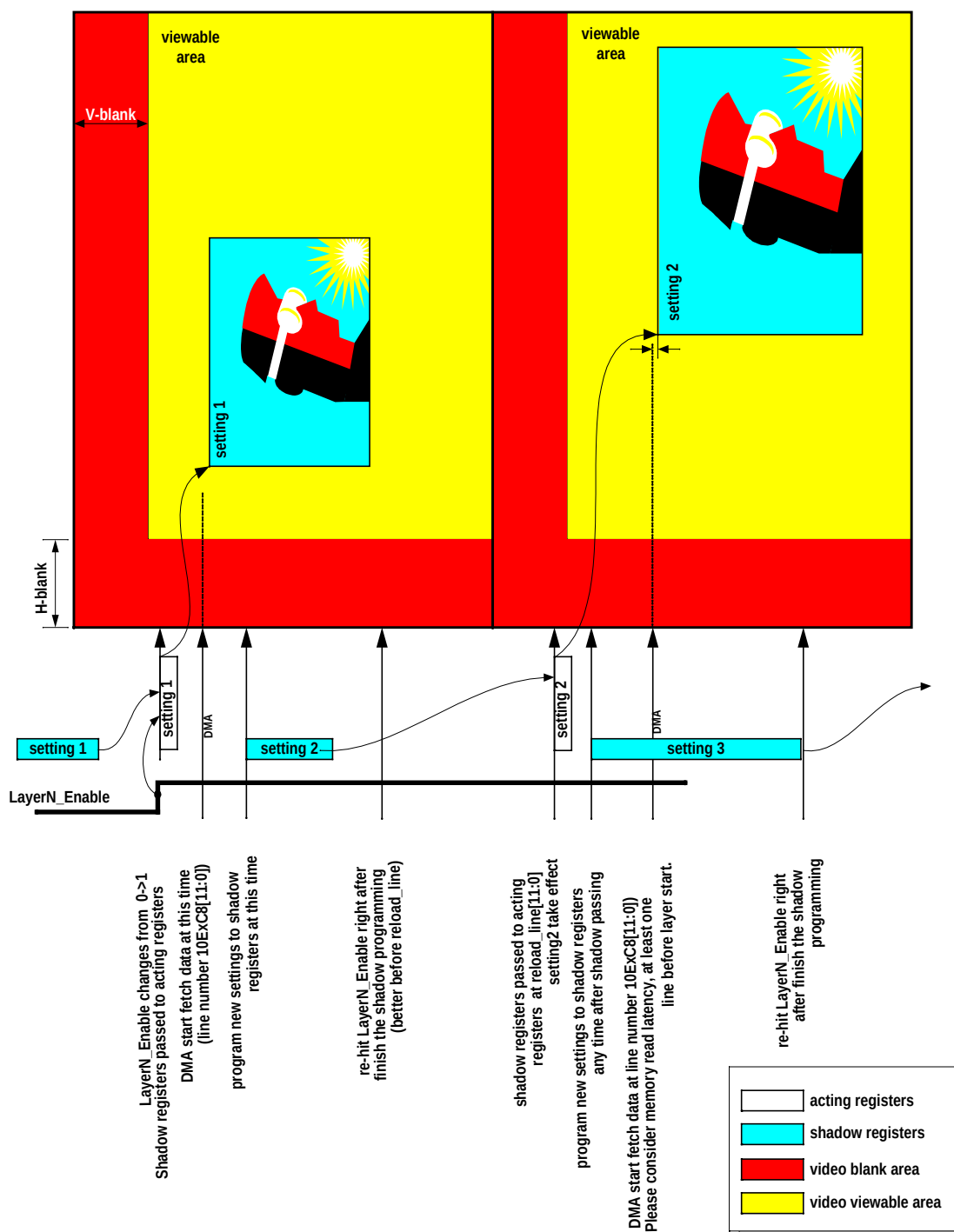
Figure 8: Shadow Mechanism
