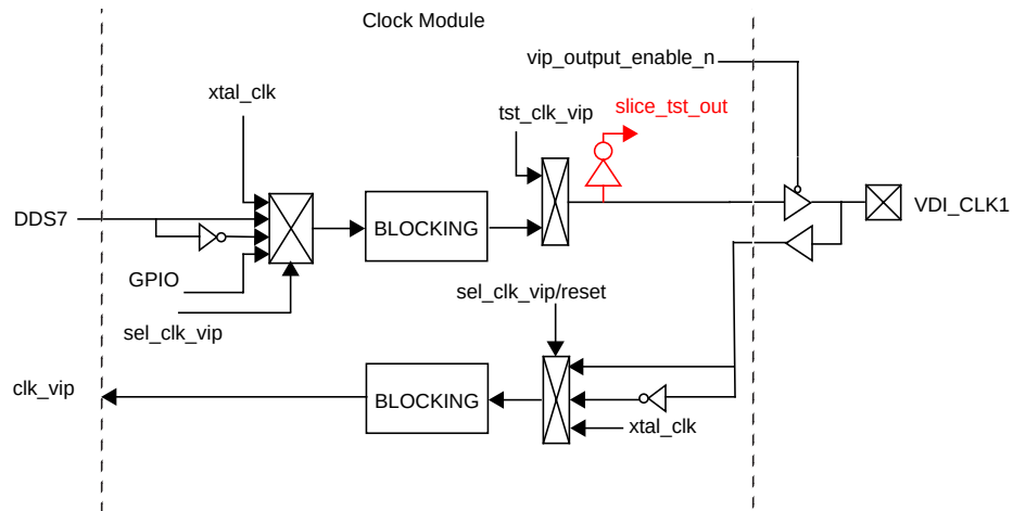
Figure 15: VDI_CLK1 Block Diagram
