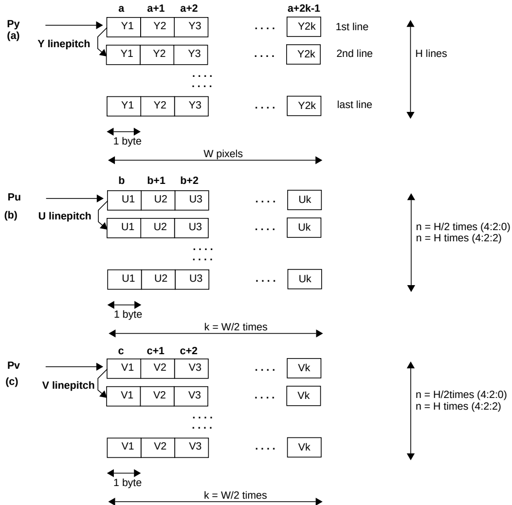
Figure 9: Planar YUV 4:2:0 and 4:2:2 Formats
