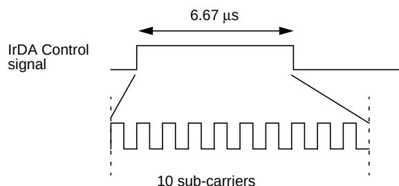
Figure 9: IrDA Control TX with Sub-Carrier Enabled
