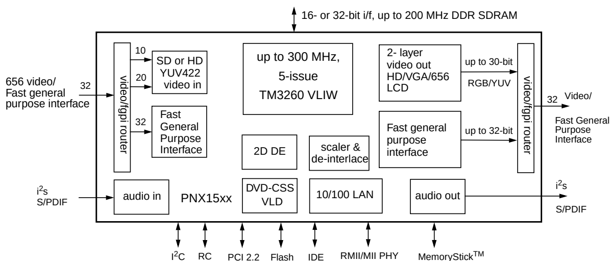
Figure 1: Block Diagram PNX15xx Series
