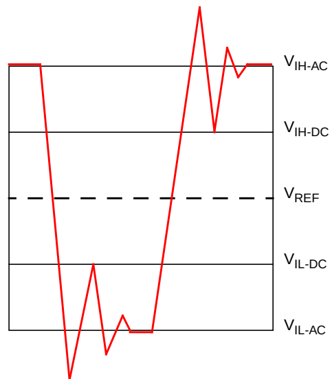
Figure 3: SSTL_2 Receiver Signal Conditions
