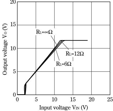
Fig.15 Output Voltage vs. Input Voltage (PQ12RD21)
