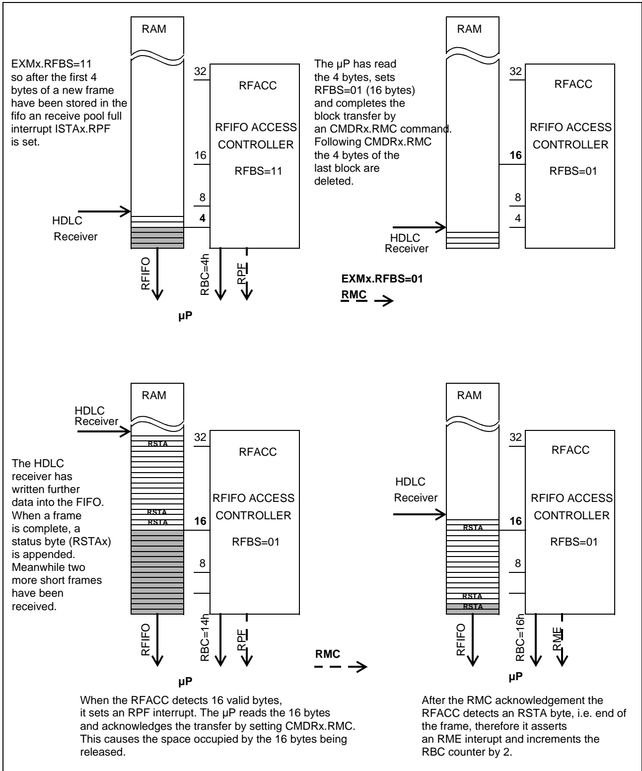
Figure 79 RFIFO Operation
