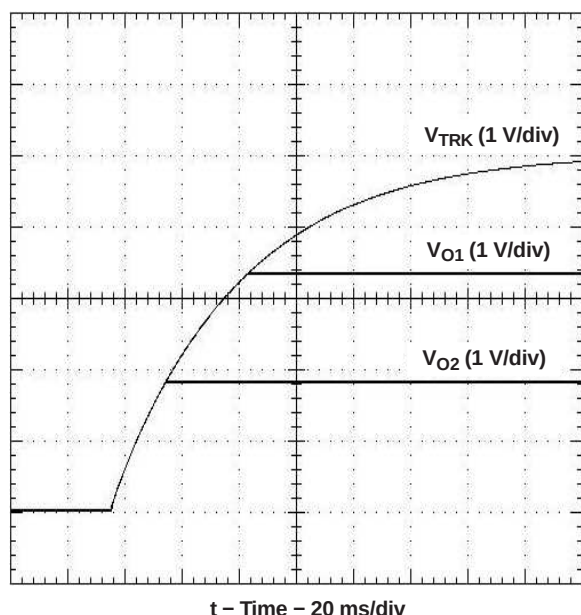
Figure 16. Simultaneous Power Up With Auto-Track Control
