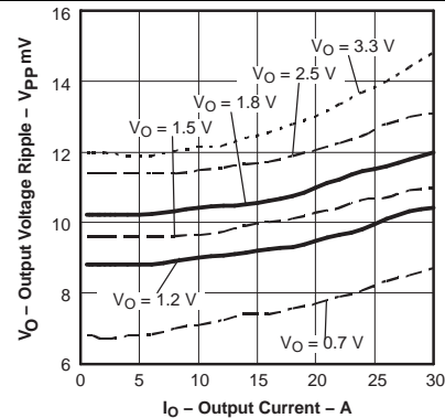
Figure 2. Output Ripple vs. Output Current
