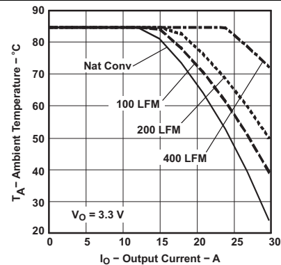
Figure 4. Ambient Temperature vs. Output Current
