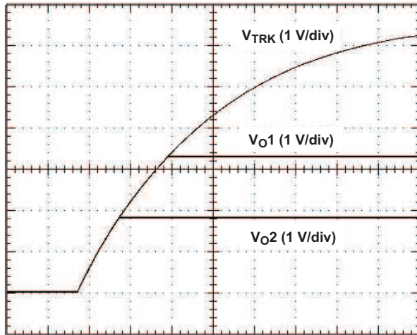
Figure 25. Simultaneous Power Up With Auto-Track Control
