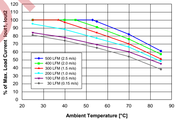
Figure 10. Available balanced load current (lout1 = 1.5·lout2) vs. ambient temperature and airflow rates for converter mounted horizontally with Vin = 48 V, air flowing from pin 3 to pin 4 and maximum FET temperature ≤ 120 °C.
