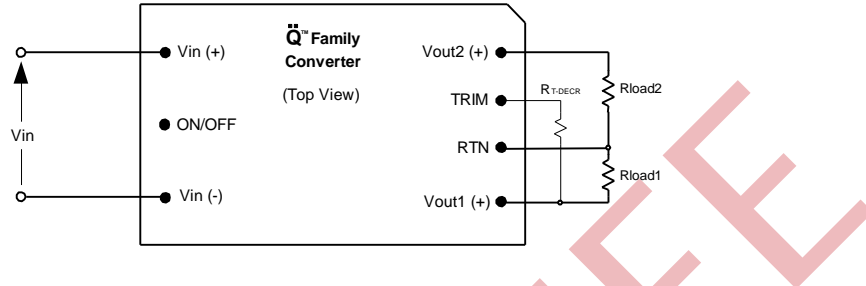
Figure 3. Configuration for decreasing output voltage.
