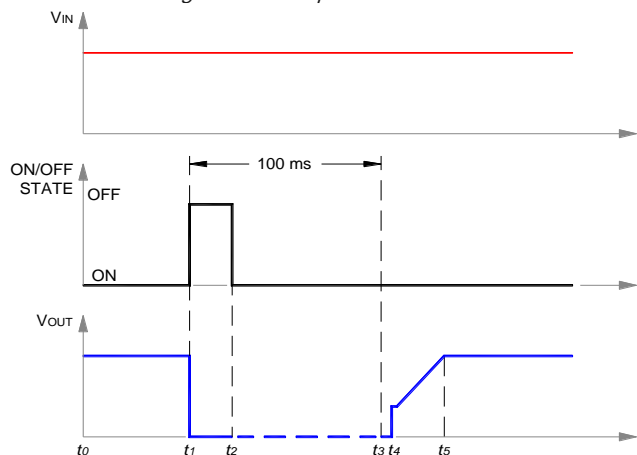
Figure 8. Startup scenario #3.
