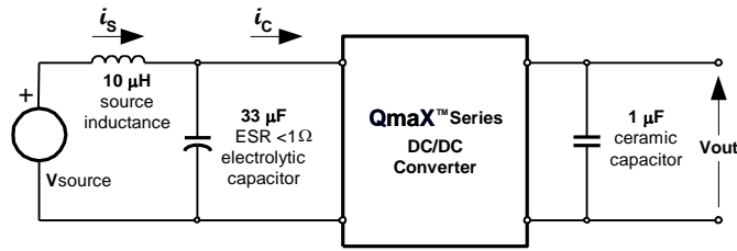
Figure 21. Test setup for measuring input reflected ripple currents, i_c and i_s .
