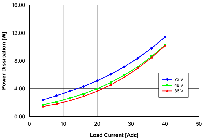
Fig. 1.5V.5: Power dissipation vs. load current and input voltage for converter mounted vertically with air flowing from pin 3 to pin 1 at a rate of 300 LFM (1.5 m/s) and T_a = 25\text{ }^\circ\text{C} .
