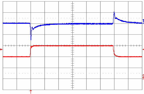
Fig. 1.8V.9: Output voltage response to load current step-change (20 A – 30 A – 20 A) at V_{in} = 48\text{ V} . Top trace: output voltage (100 mV/div.). Bottom trace: load current (10 A/div). Current slew rate: 1 A/ \mu\text{s} . C_o = 470\text{ }\mu\text{F} tantalum + 1 \mu\text{F} ceramic. Time scale: 0.2 ms/div.
