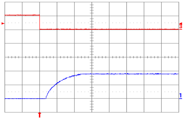
Figure 1.8V.16. Turn-on transient at full rated load current (resistive) plus 10,000 \mu\text{F} at V_{in} = 48\text{ V} , triggered via ON/OFF pin. Top trace: ON/OFF signal (5 V/div.). Bottom trace: output voltage (1 V/div.). Time scale: 2 ms/div.
