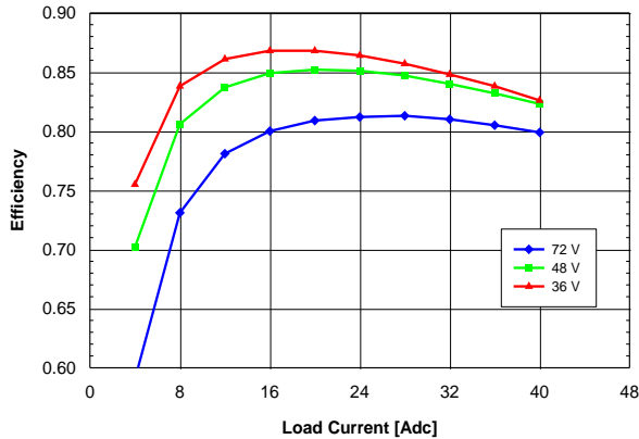
Figure 1.2V.11. Efficiency vs. load current and input voltage for QME48T40012 converter mounted horizontally with air flowing from pin 1 to pin 3 at a rate of 300 LFM (1.5 m/s) and T_a = 25\text{ }^{\circ}\text{C} .
