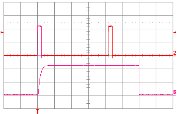
Figure 1.8V.24. Load current (top trace, 20 A/div., 50 ns/div.) into a 10 \text{ m}\Omega short circuit during restart, at V_{in} = 48 \text{ V} . Bottom trace (20 A/div., 2 ns/div.) is an expansion of the on-time portion of the top trace.
