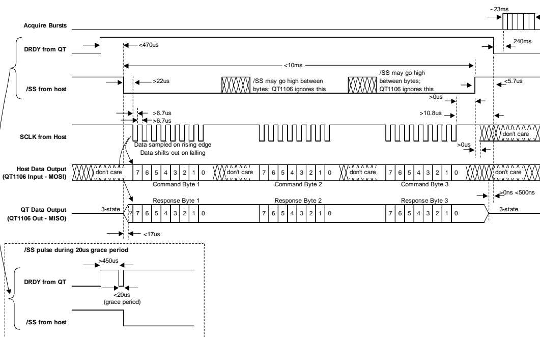
Figure 3.1 SPI Operation
