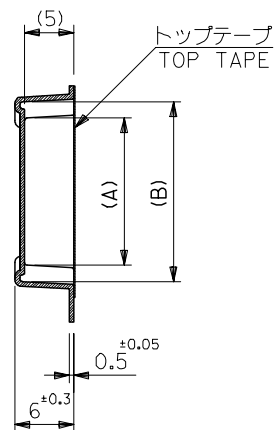
SECT:Y-Y
