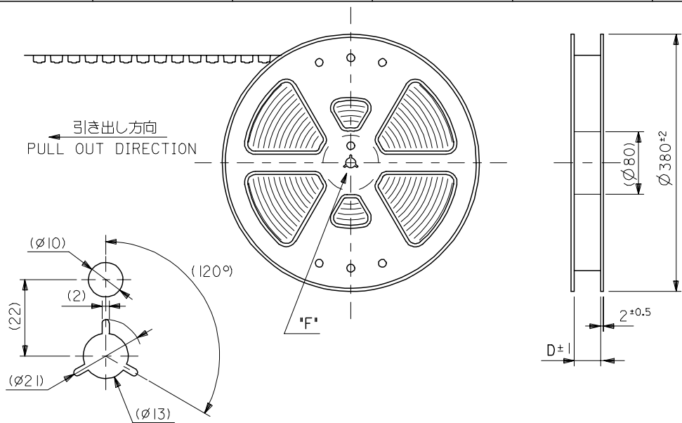
DETAIL "F"
