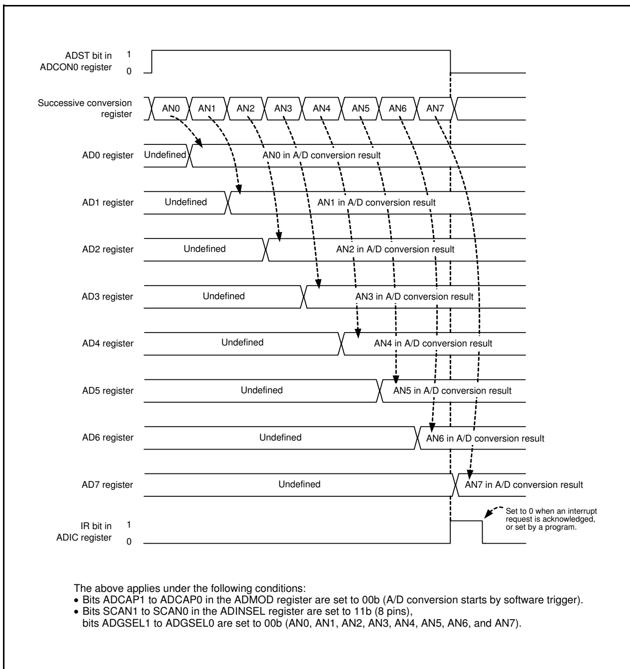
Figure 29.8 Operating Example in Single Sweep Mode
