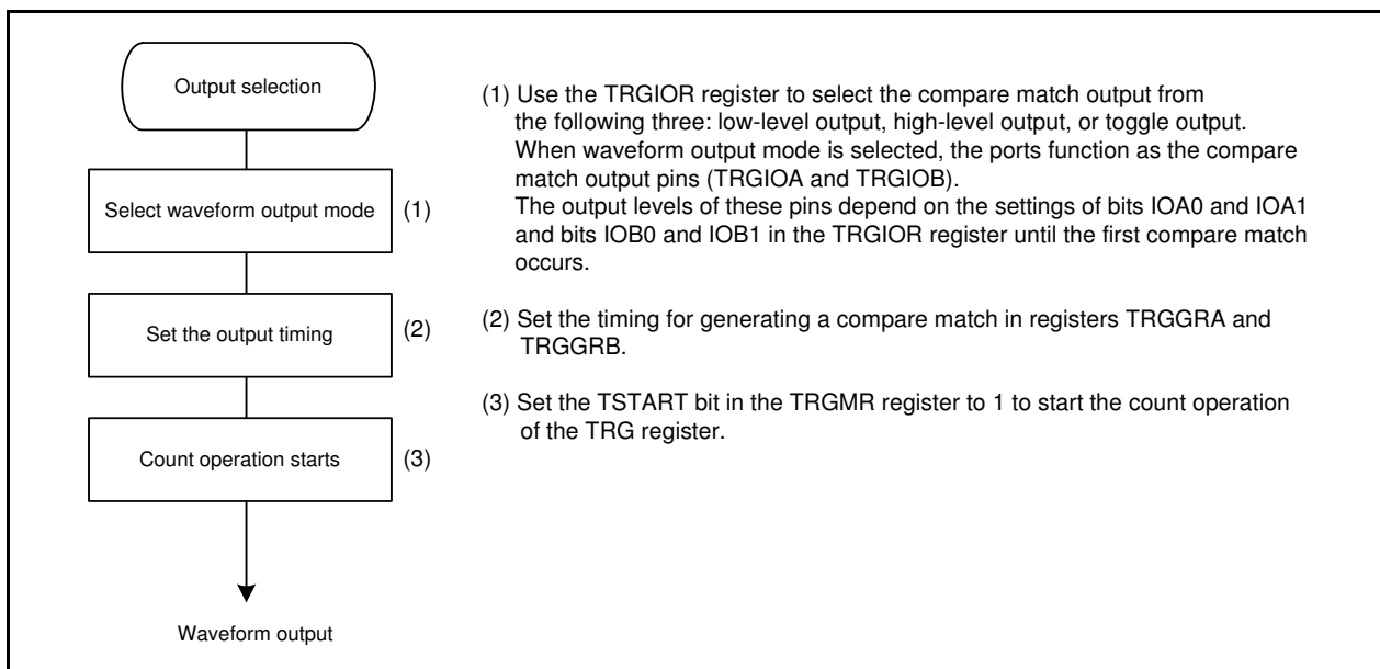
Figure 22.9 Operating Example of Waveform Output by Compare Match
