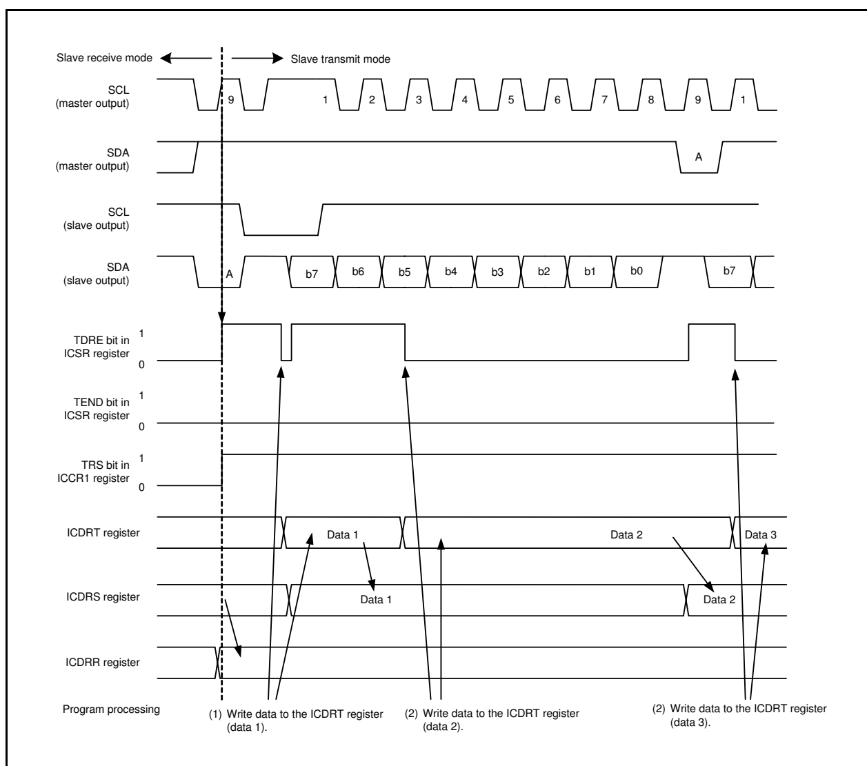
Figure 27.9 Operating Timing in Slave Transmit Mode (I 2 C bus Interface Mode) (1)
