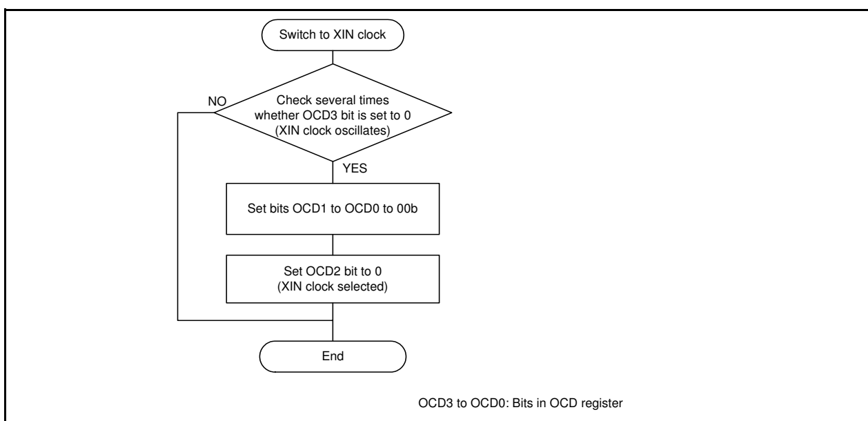
Figure 8.5 Procedure for Switching Low-Speed On-Chip Oscillator to XIN Clock
