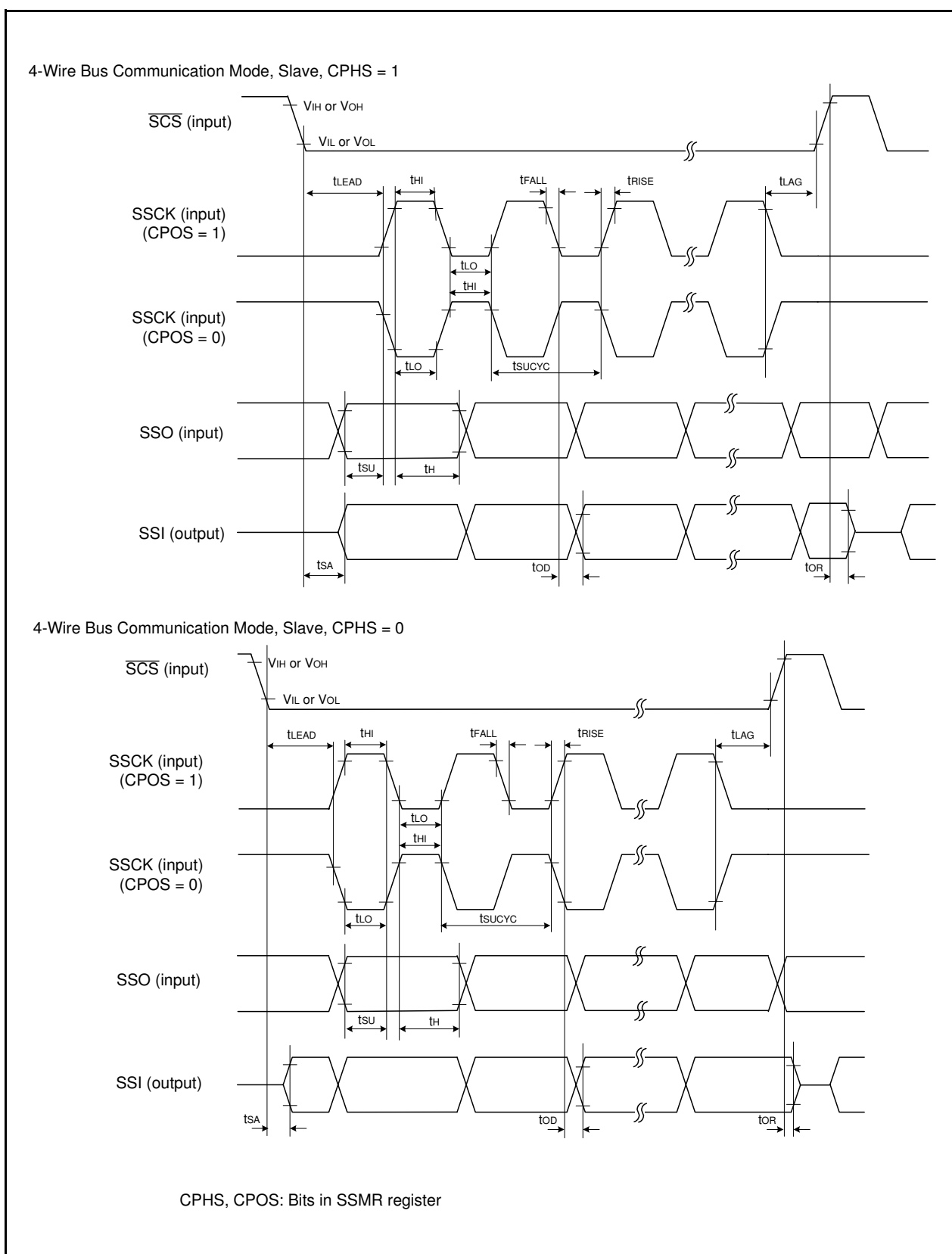
Figure 34.4 I/O Timing of Clock Synchronous Serial I/O with Chip Select (Slave)
