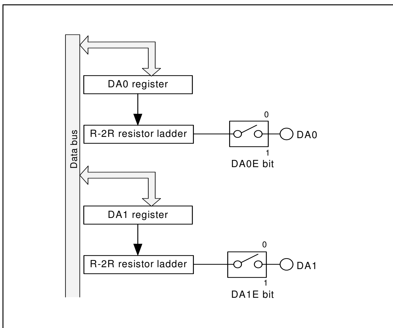
Figure 30.1 D/A Converter Block Diagram
