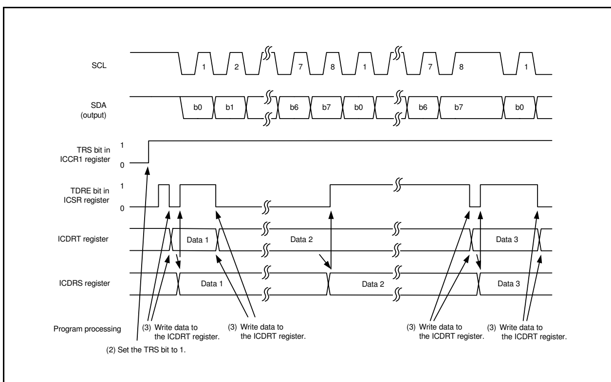
Figure 27.14 Operating Timing in Transmit Mode (Clock Synchronous Serial Mode)
