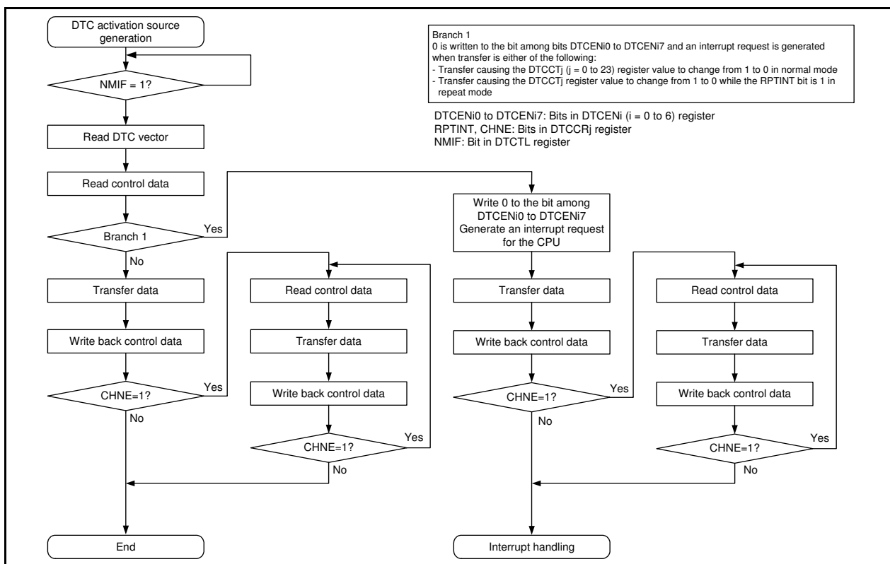
Figure 15.3 DTC Internal Operation Flowchart When DTC Activation Source is not SSU/I²C bus, Timer RC, Timer RD, Timer RG, or Flash Memory Interrupt Source
