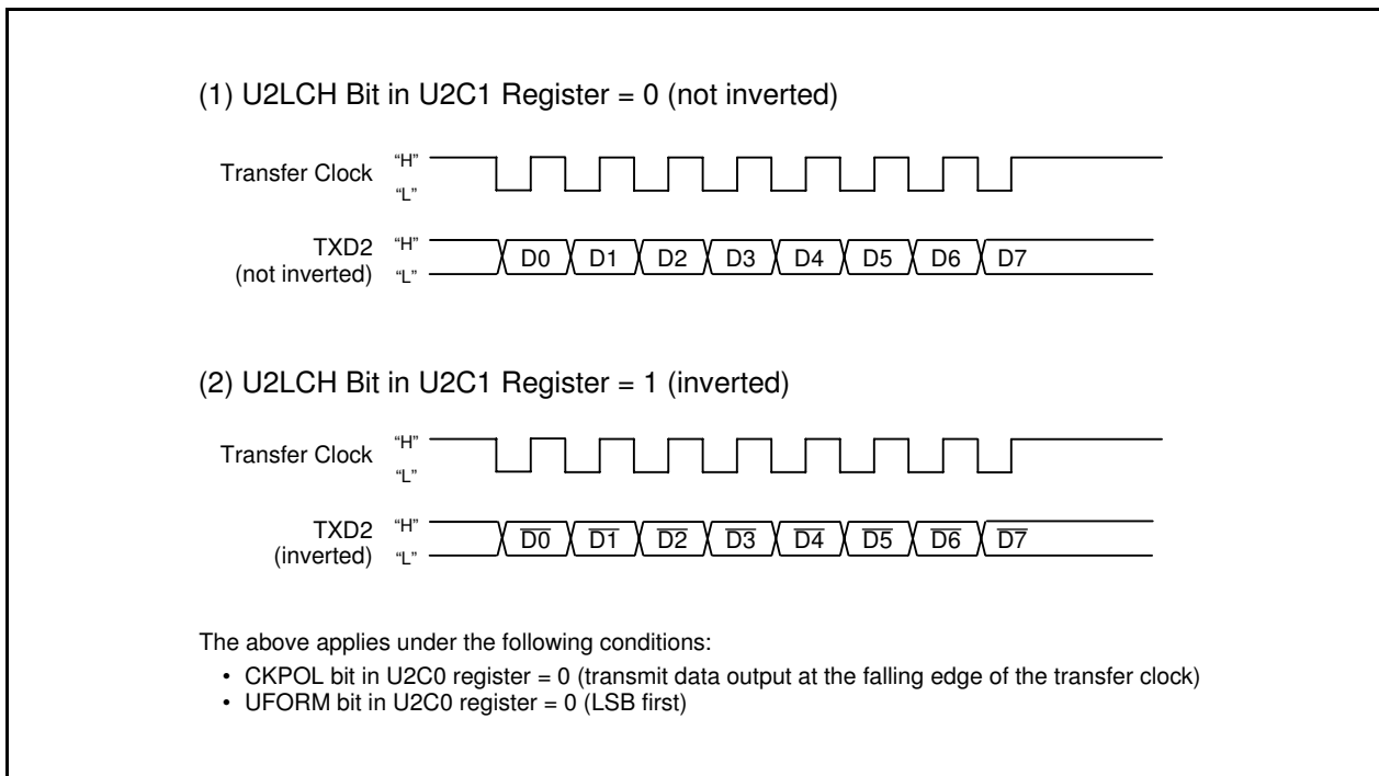
Figure 24.6 Serial Data Logic Switching
