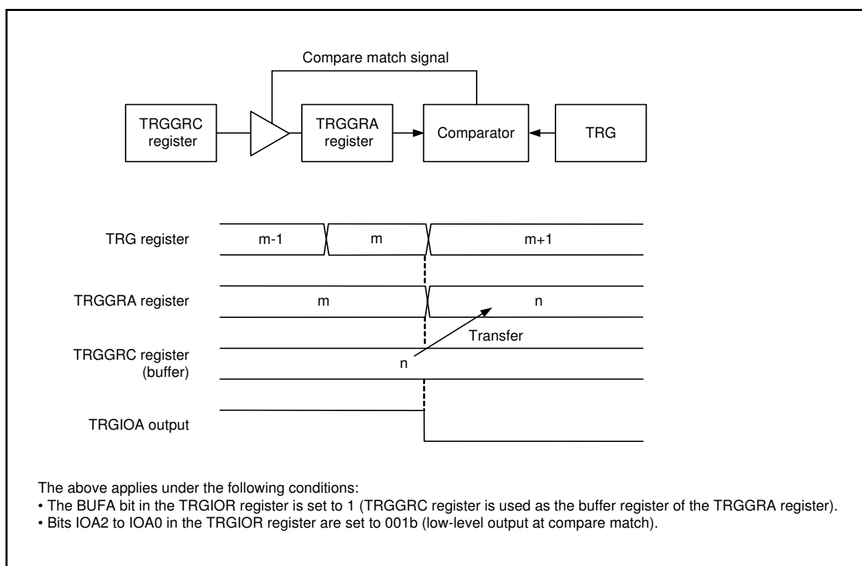
Figure 22.4 Buffer Operation of Output Compare Function
