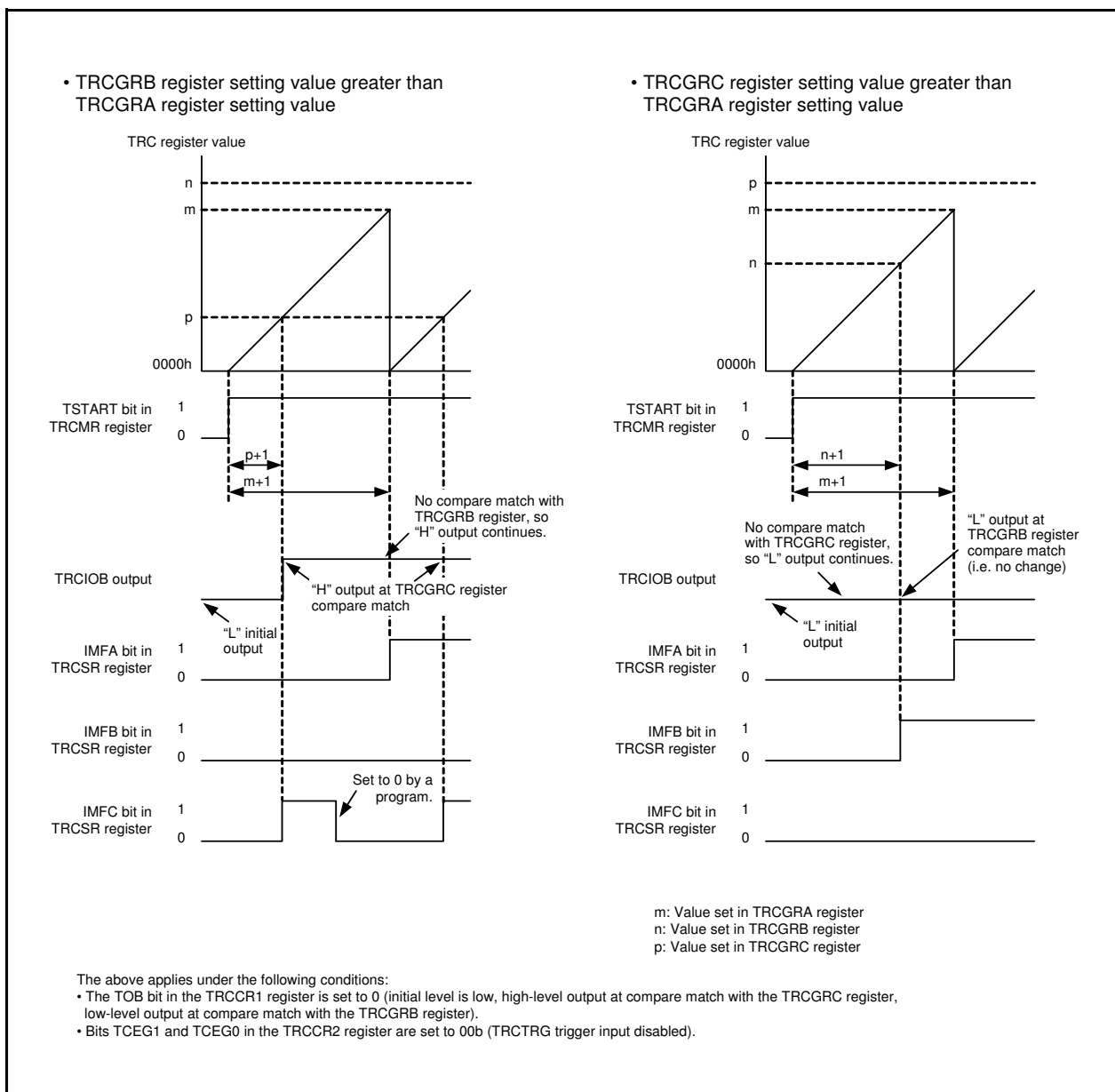
Figure 19.19 Operating Example in PWM2 Mode (Duty 0% and Duty 100%)
