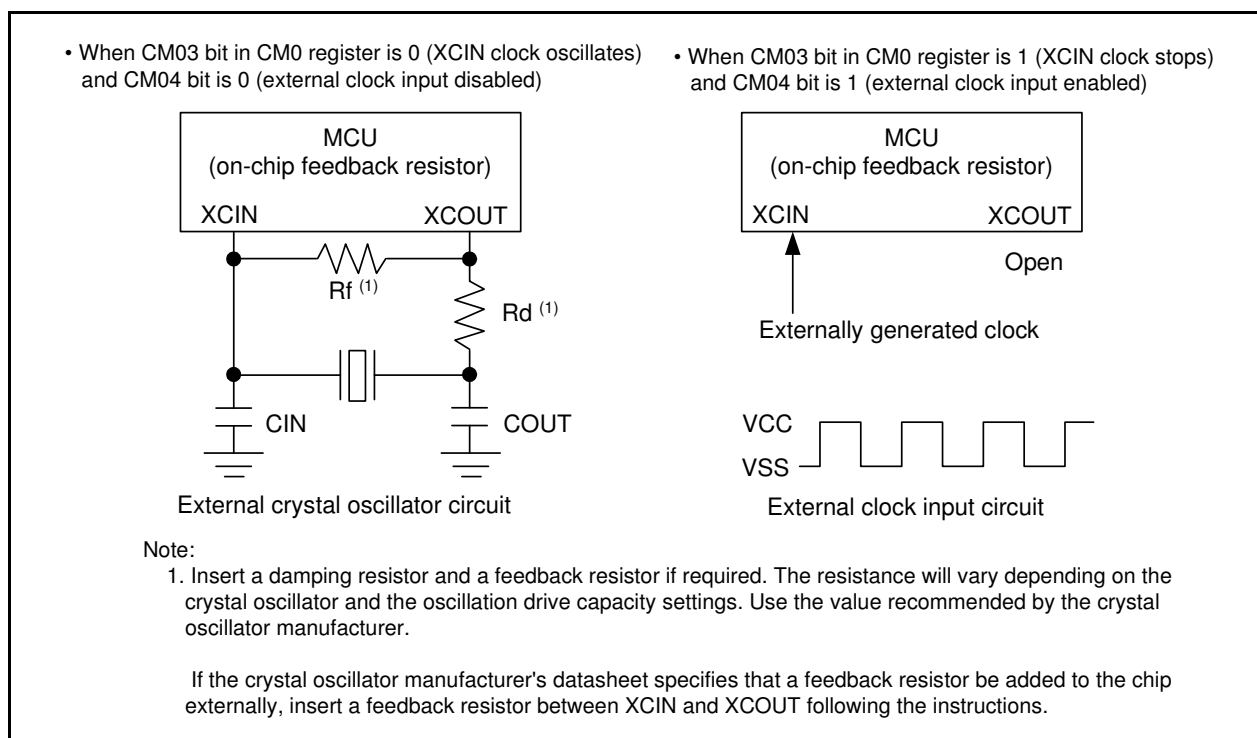
Figure 8.4 Examples of XCIN Clock Connection Circuits
