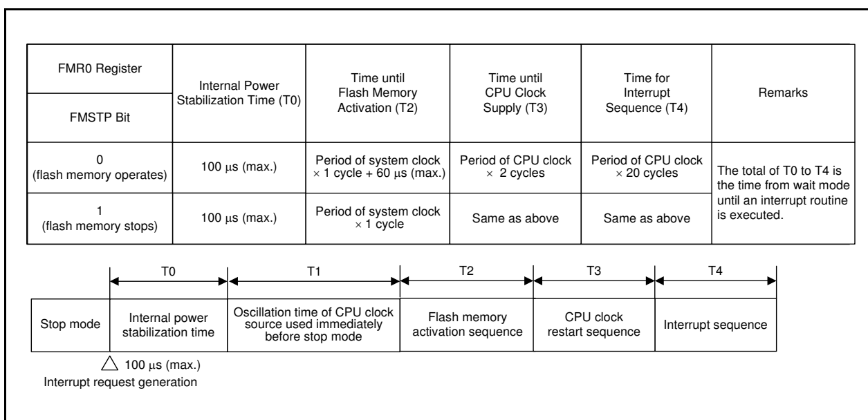
Figure 9.4 Time from Stop Mode to Interrupt Routine Execution
