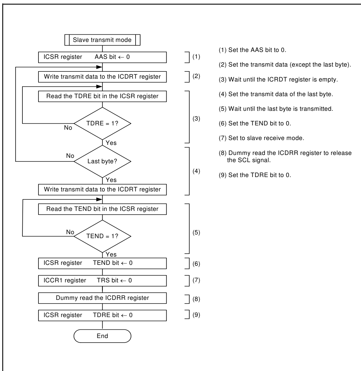
Figure 27.18 Register Setting Example in Slave Transmit Mode (I 2 C bus Interface Mode)
