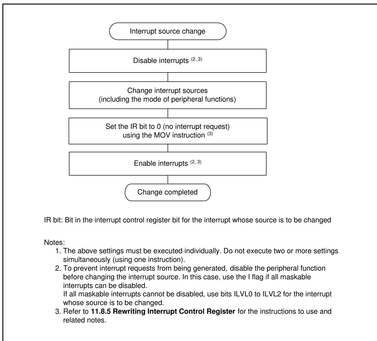
Figure 35.1 Procedure Example for Changing Interrupt Sources
