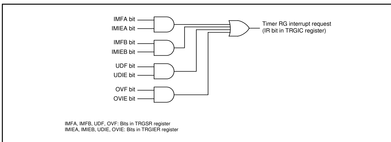
Figure 22.21 Block Diagram of Timer RG Interrupt
