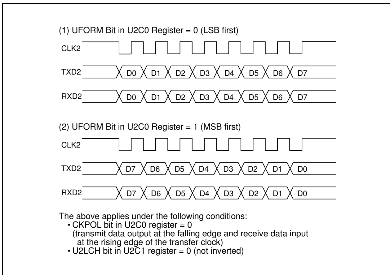
Figure 24.5 Transfer Format
