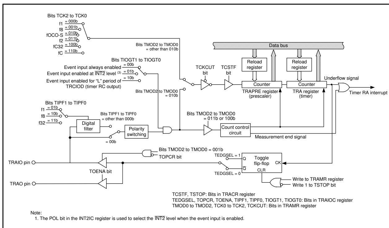
Figure 17.1 Timer RA Block Diagram
