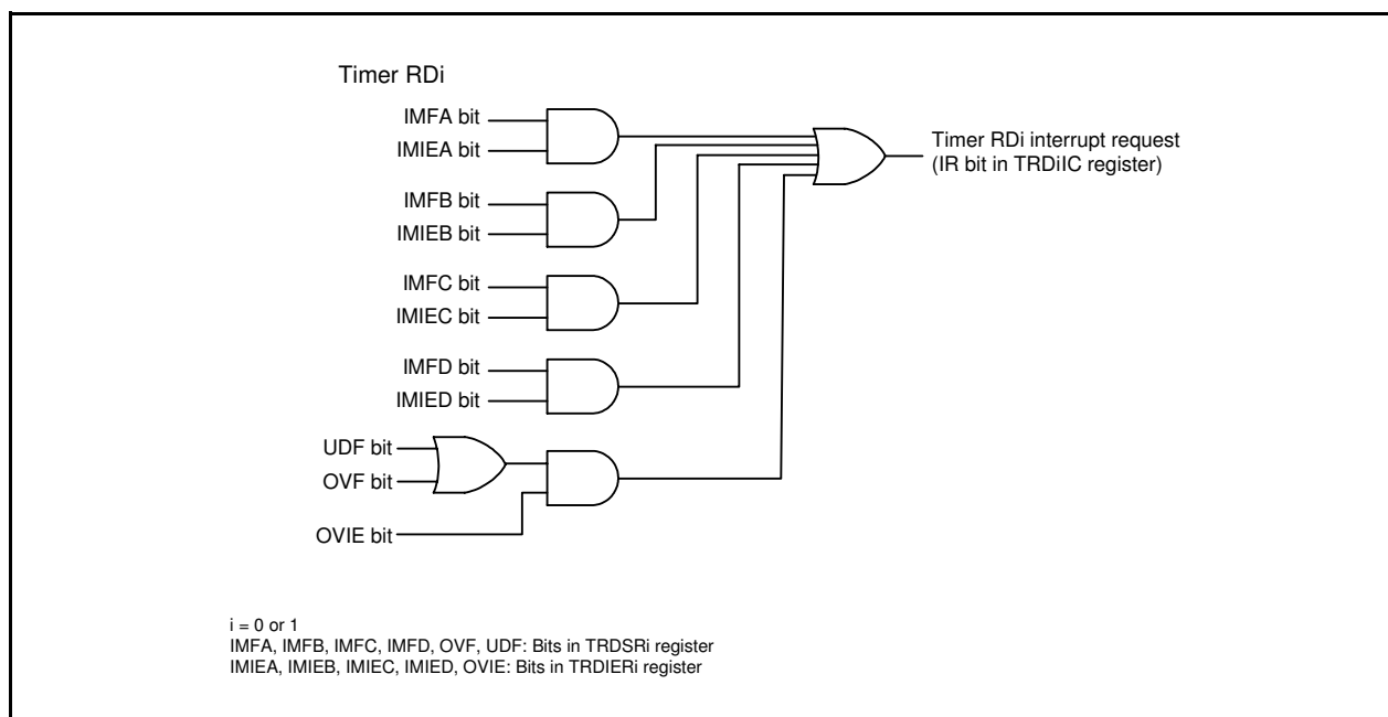
Figure 11.12 Block Diagram of Timer RD Interrupt
