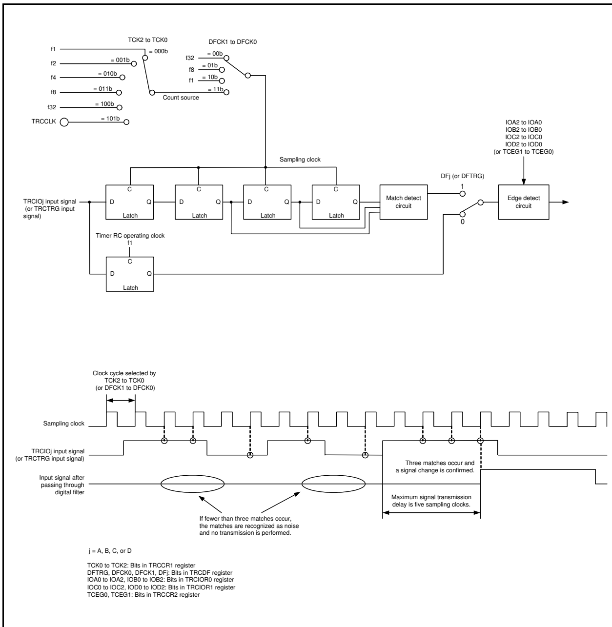
Figure 19.5 Block Diagram of Digital Filter
