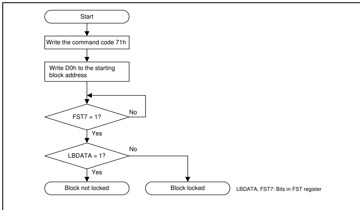
Figure 33.13 Read Lock Bit Status Flowchart
