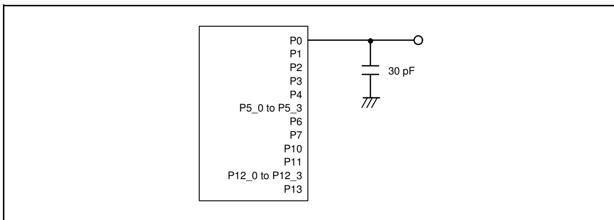
Figure 34.1 Ports P0 to P4, P5_0 to P5_3, P6, P7, P10, P11, P12_0 to P12_3, and P13 Timing Measurement Circuit
