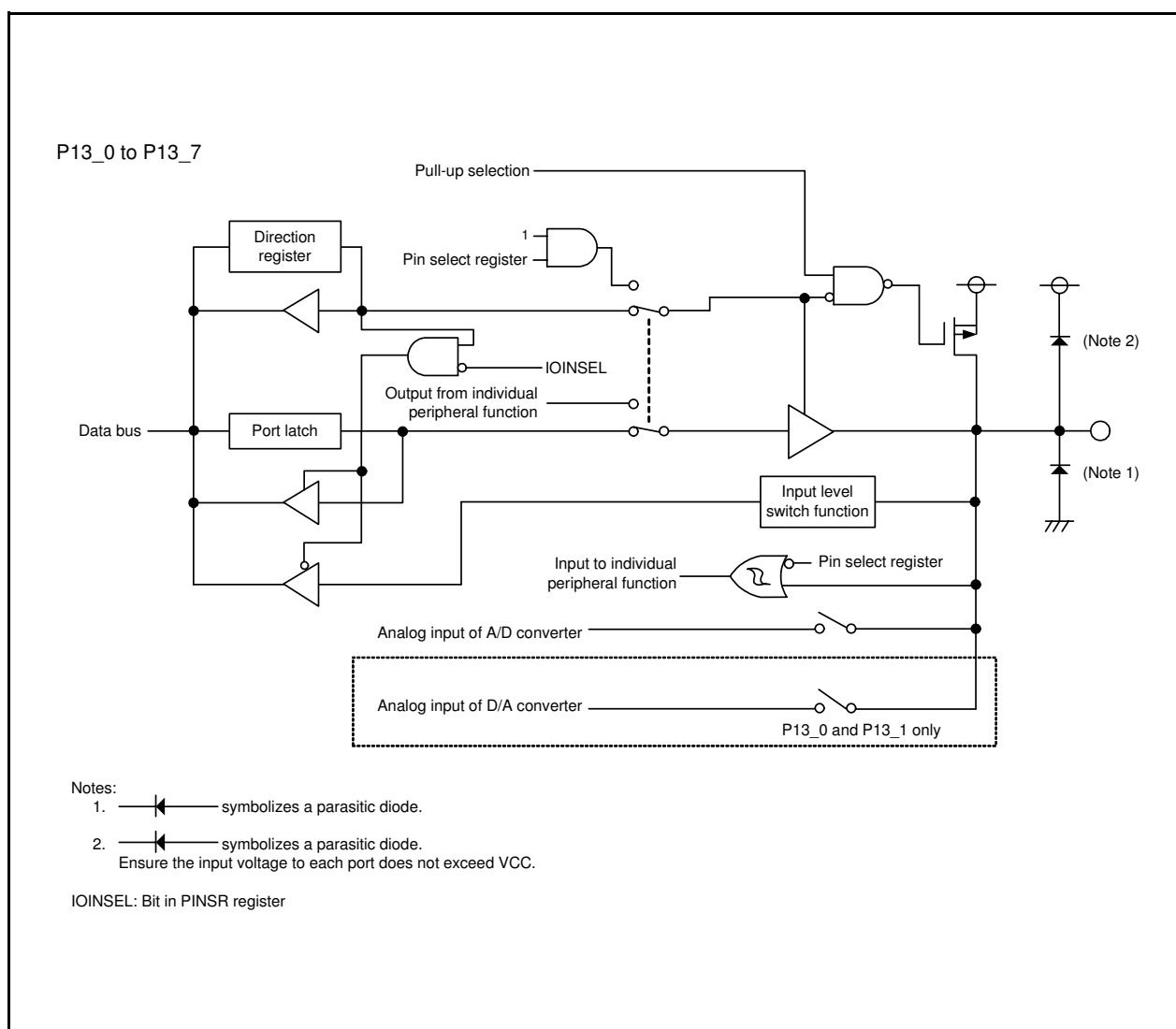
Figure 6.4 I/O Port Configuration (4)
