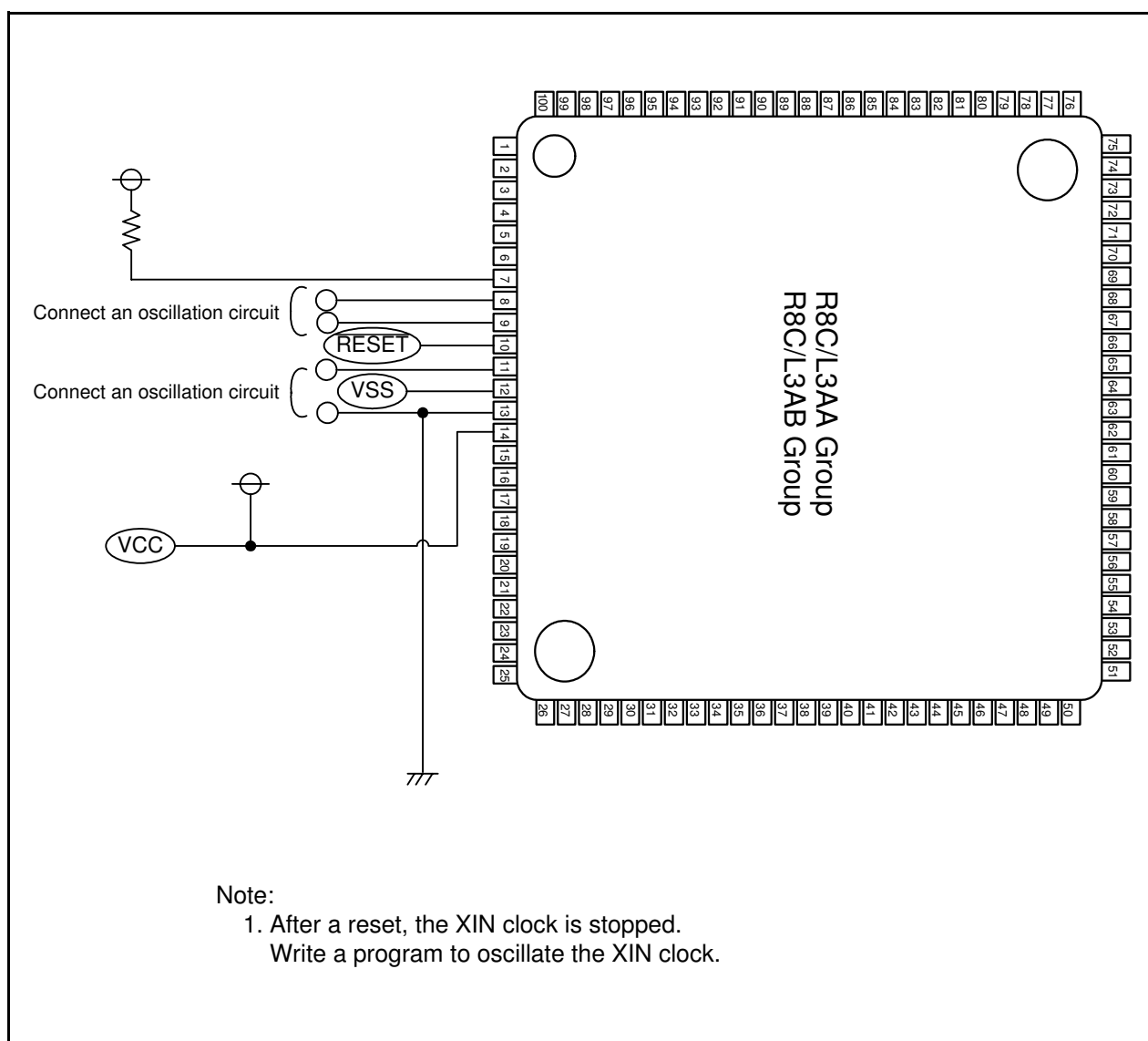
Appendix Figure 4.4 Example of Oscillation Evaluation Circuit (4)
