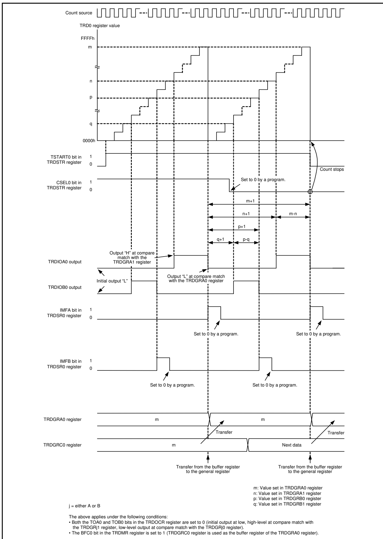
Figure 20.23 Operating Example in PWM3 Mode
