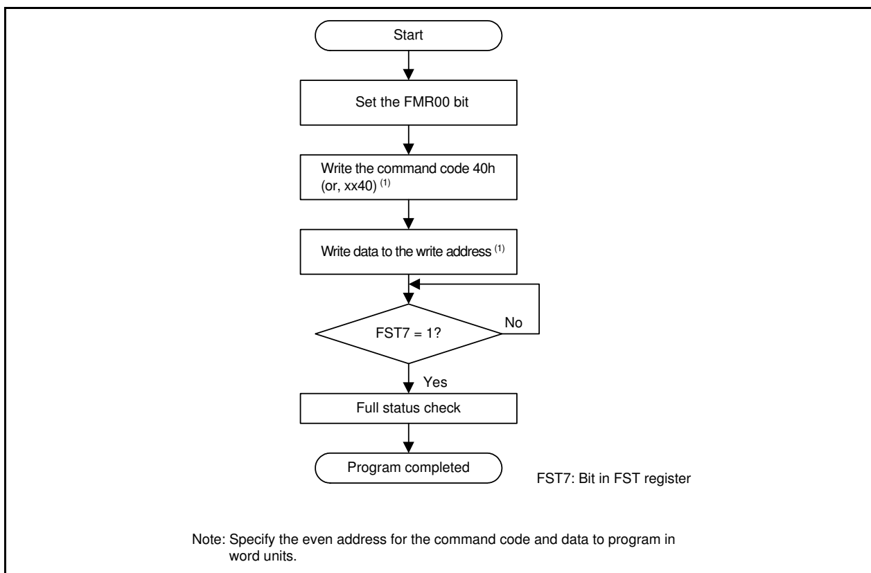
Figure 33.7 Program Flowchart (Flash Ready Status Interrupt Disabled)
