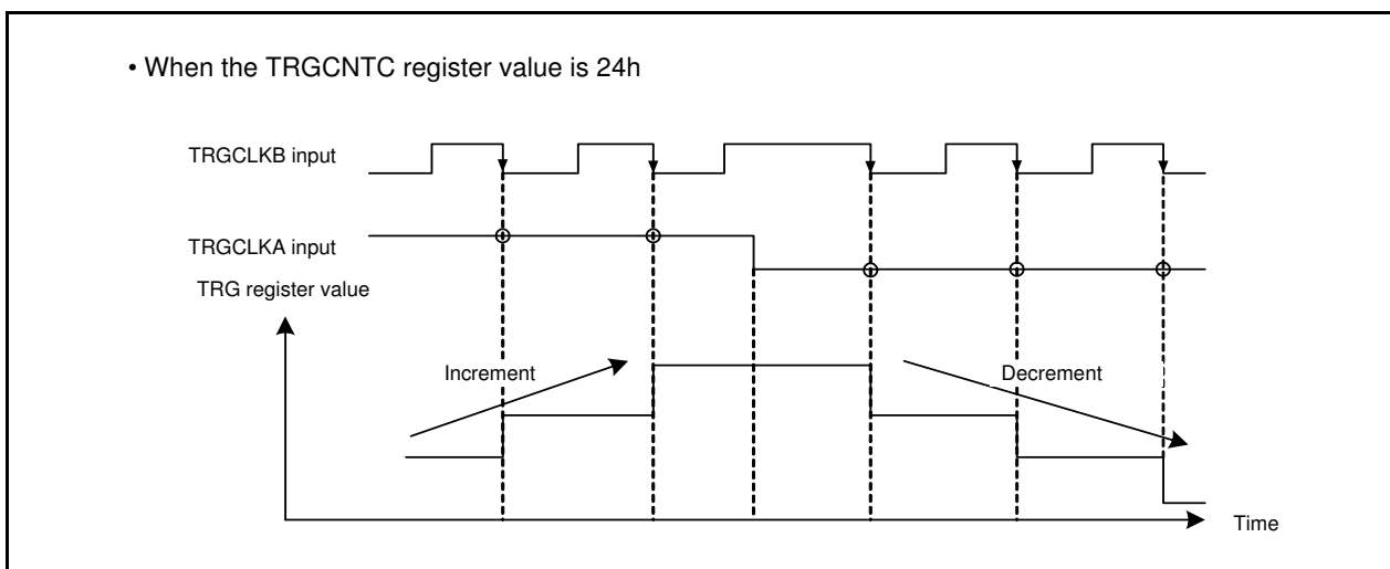
Figure 22.18 Operating Example in Phase Counting Mode 2
