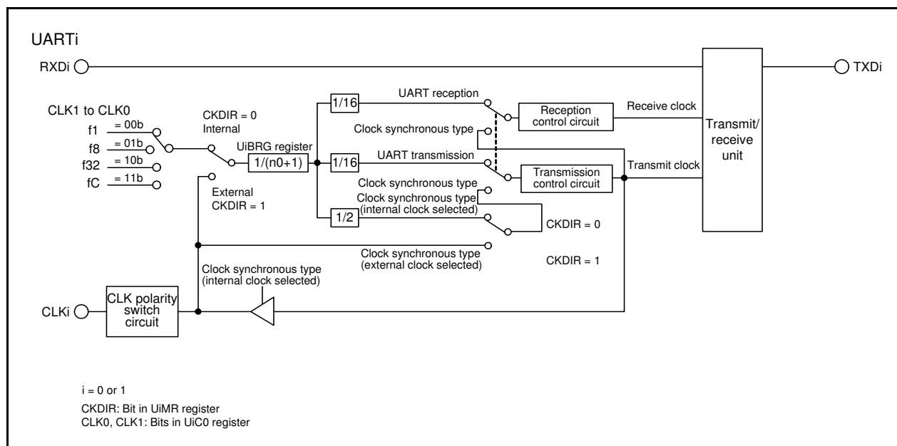
Figure 23.1 Block Diagram of UARTi (i = 0 or 1)
