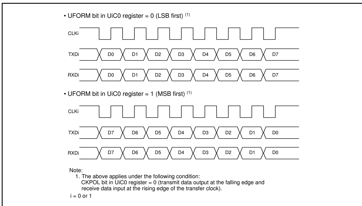
Figure 23.5 Transfer Format
