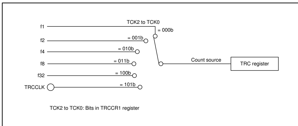
Figure 19.2 Count Source Block Diagram
