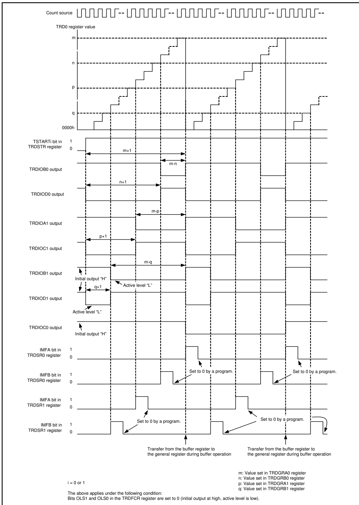
Figure 20.18 Operating Example in Reset Synchronous PWM Mode
