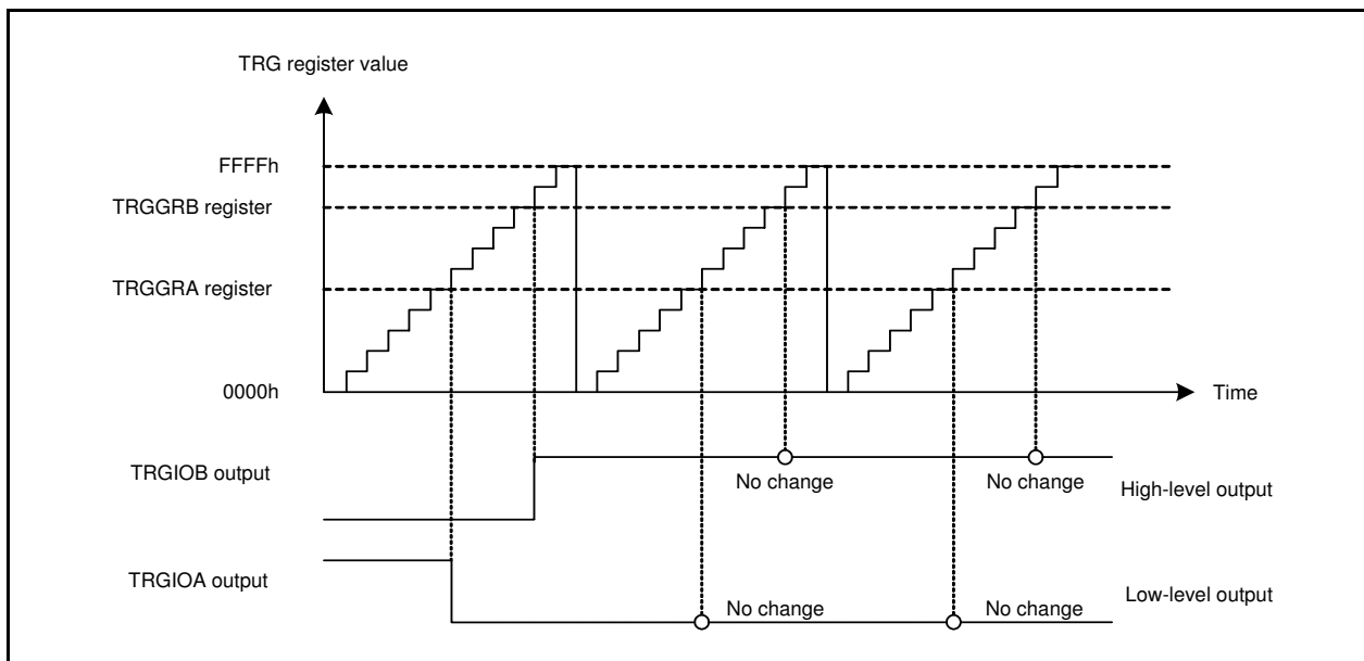
Figure 22.11 Operating Example of Low-Level Output and High-Level Output
