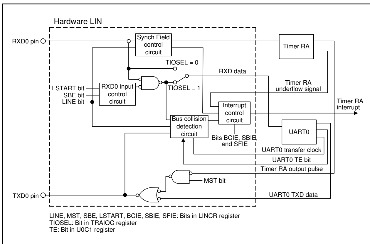
Figure 28.1 Hardware LIN Block Diagram
