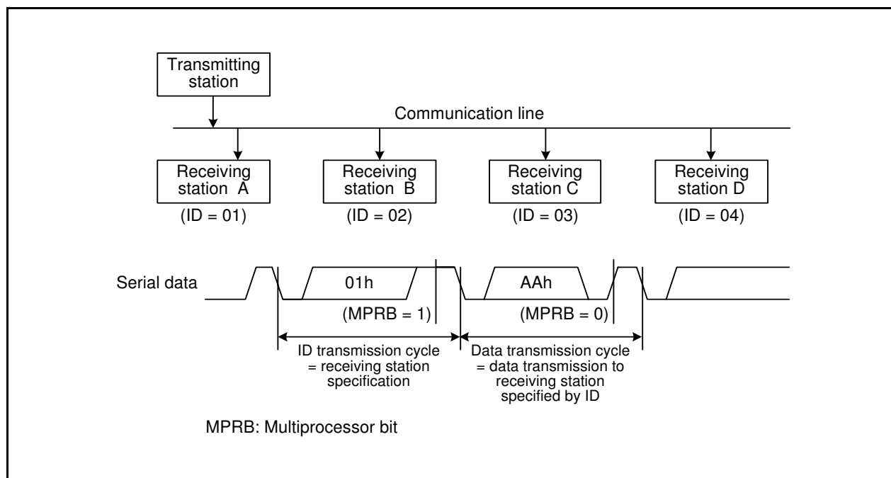
Figure 24.17 Multiprocessor Communication Example Using Multiprocessor Format (Data AAh Transmission to Receiving Station A)
