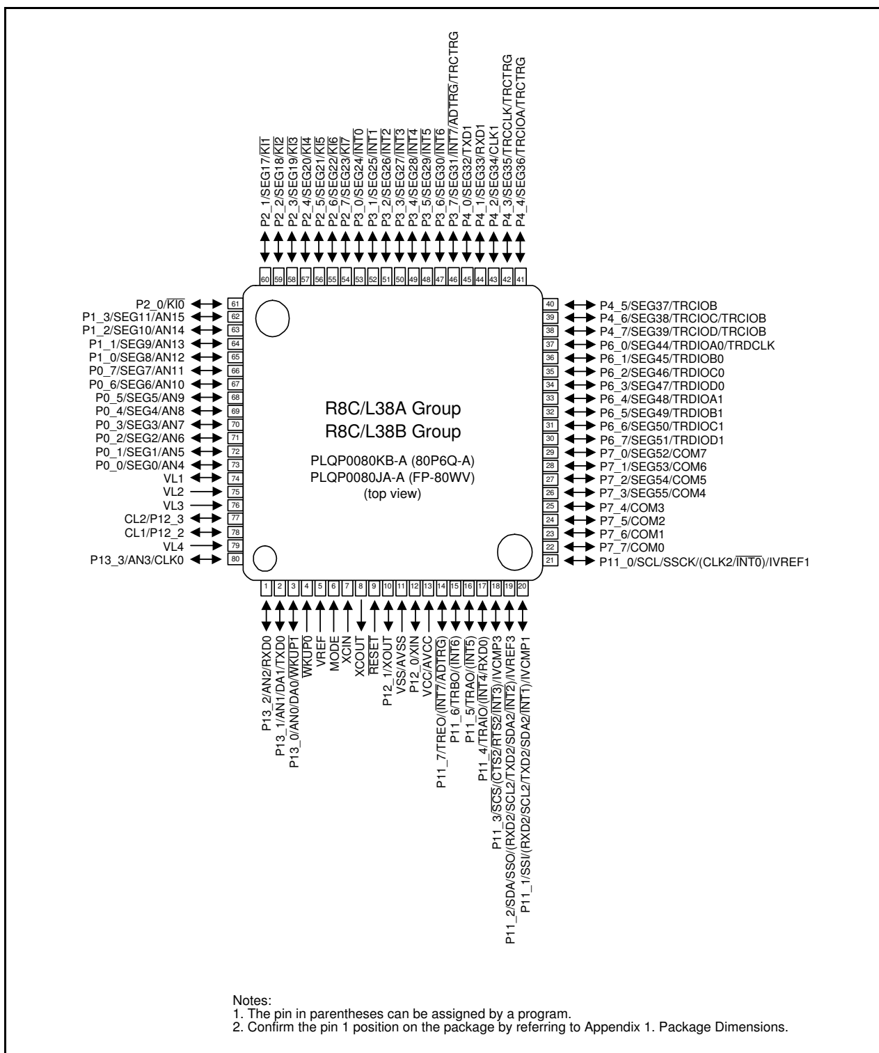
Figure 1.15 Pin Assignment (Top View) of PLQP0080KB-A and PLQP0080JA-A Packages
