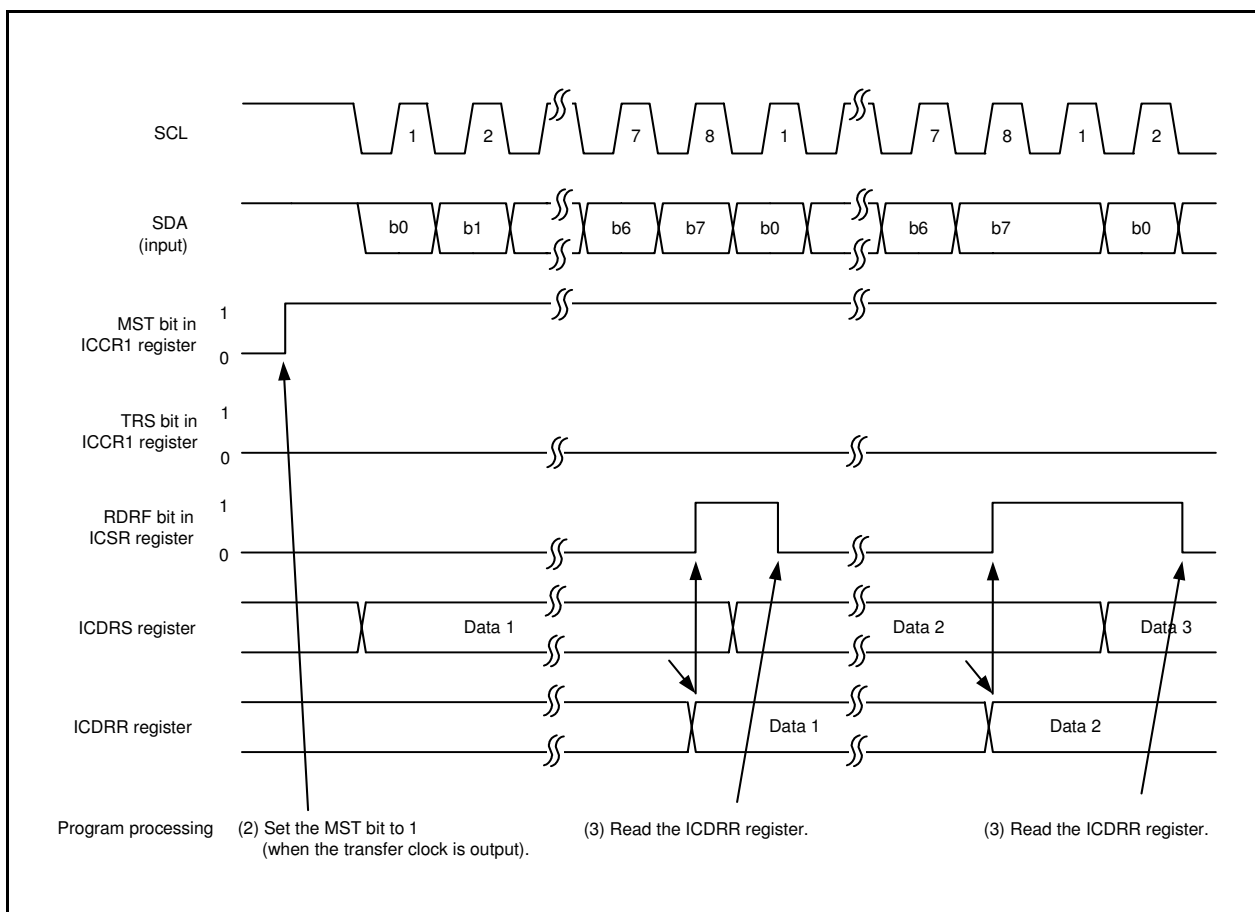
Figure 27.15 Operating Timing in Receive Mode (Clock Synchronous Serial Mode)
