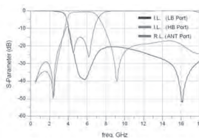
RFDIP1608060LVT
