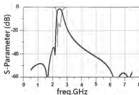
RFBPF2520080AUT
