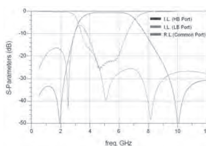
RFDIP1607L898D1T
