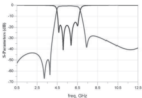
RFBPF1608060KG8D1T
