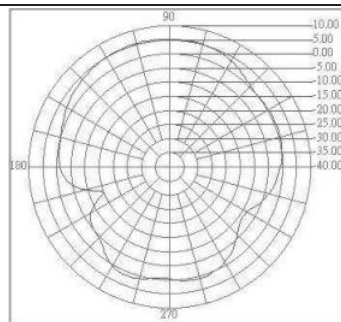
X-Y Plane Horizontal
