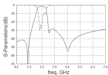
RFBPF1608070AWT
