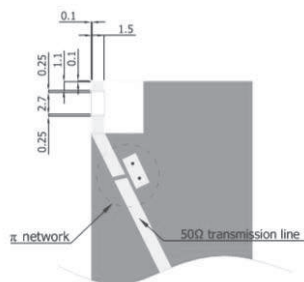
Land Pattern
