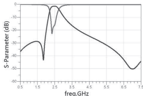
RFBPF1608060A1T
