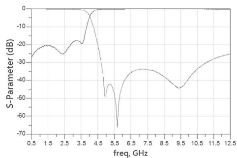
RFLPF16082G6W2T
