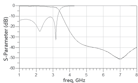
RFLPF1608060AAT
