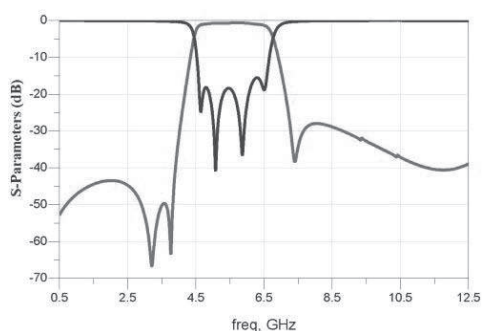
RFBPF2012090K5T
