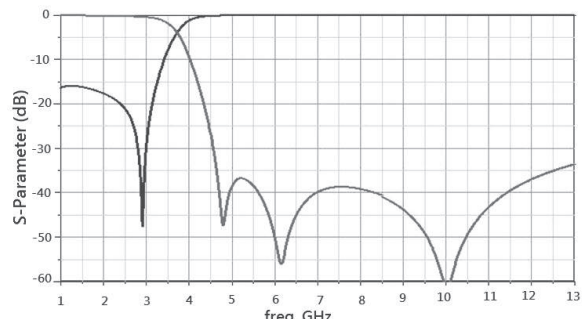
RFLPF16082G5WM0T29
