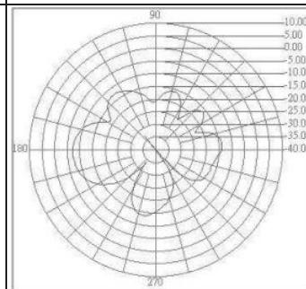
Y-Z Plane Horizontal
