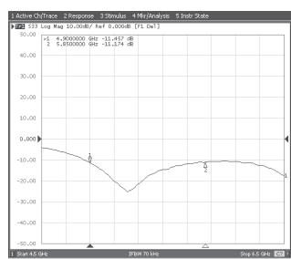
Return Loss (S11)
