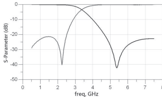
RFLPF1005040A2T
