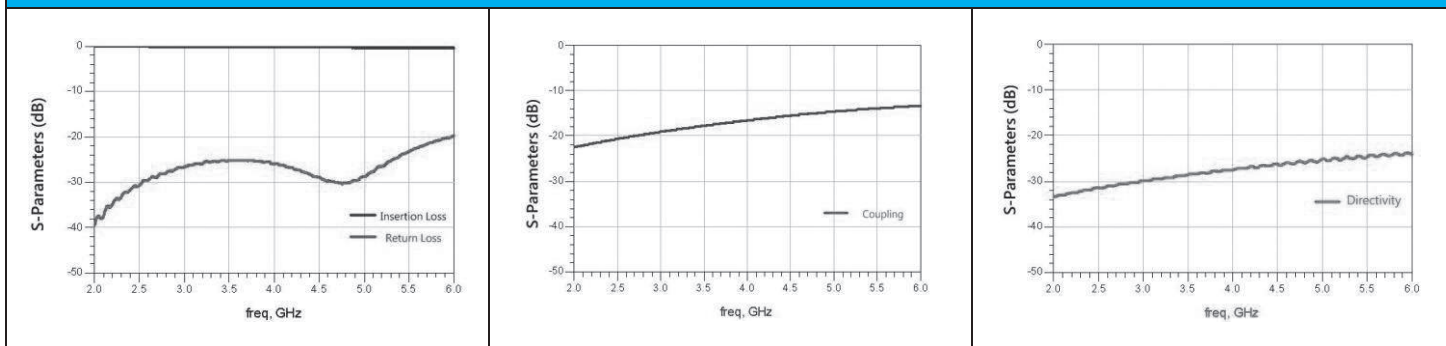
RFCPL0605030L9T
