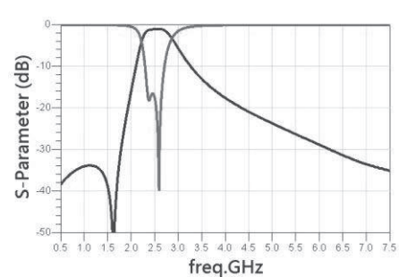
RFBPF1608050A0T
