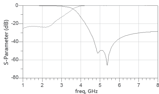
RFLPF2012090BM0T29
