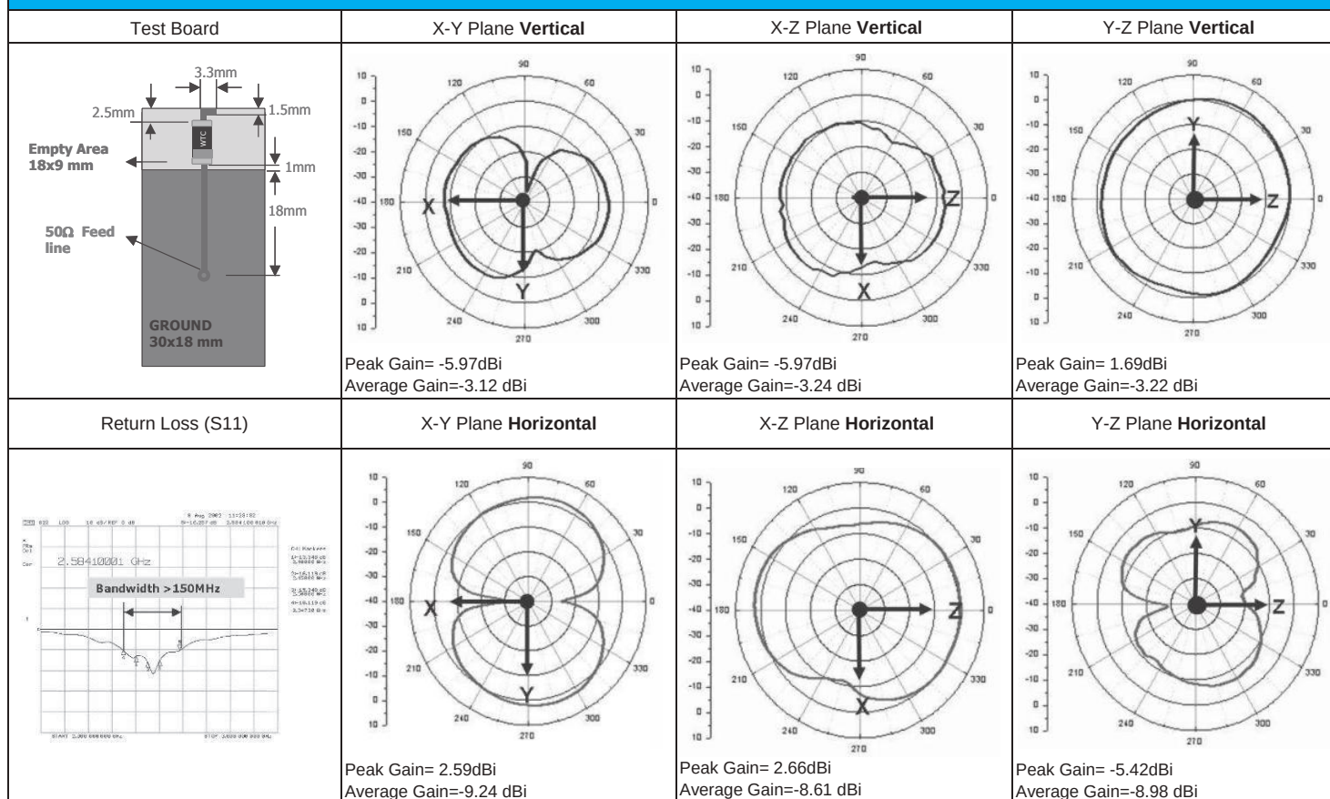
RGFAR1903041A1T
