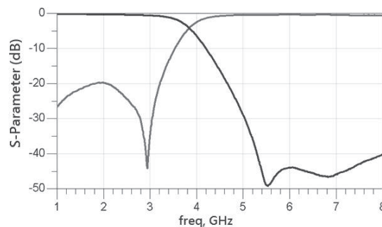
RFLPF16082G5W0T
