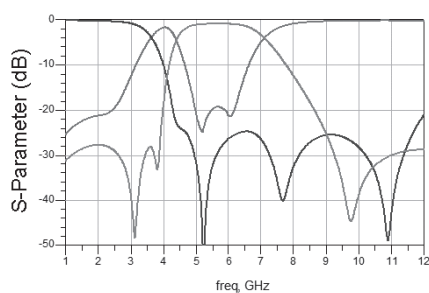
RFDIP1606L168M1U
