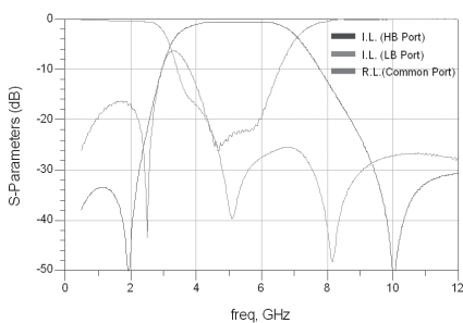
RFDIP1606L53T
