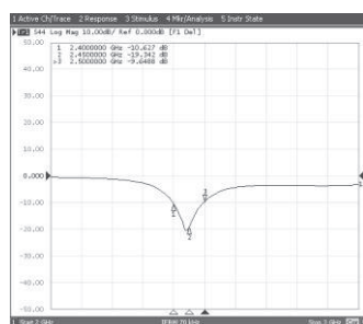
Return Loss (S11)
