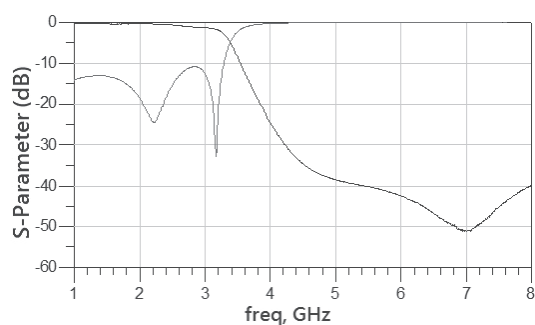
RFLPF1608060AM2T66
