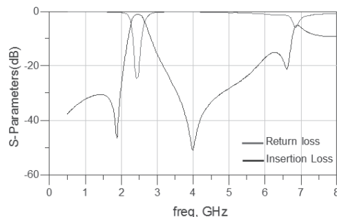
RFBPF2012100A6T
