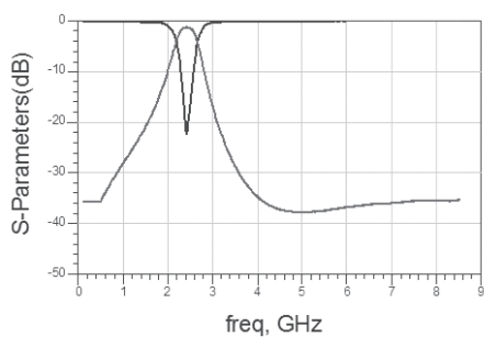
RFBPF1608070AFT
