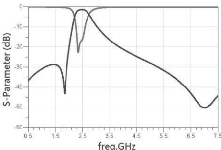
RFBPF1608060A1T
