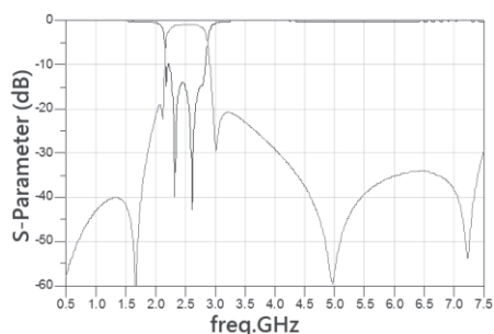
RFBPF2012090A1T
