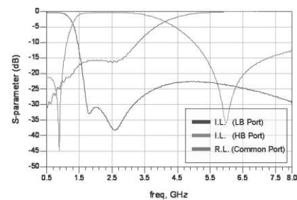
RFDIP2520100G2T
