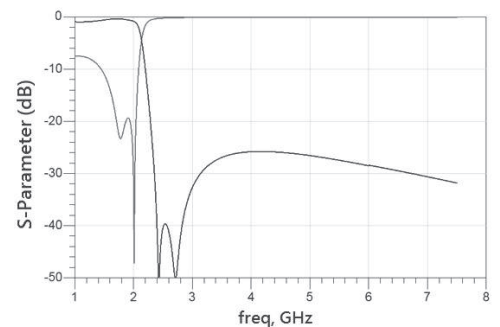
RFLPF1005040A1T
