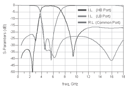
RFDIP1606L168M1U
