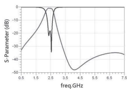
RFBPF1608060AET
