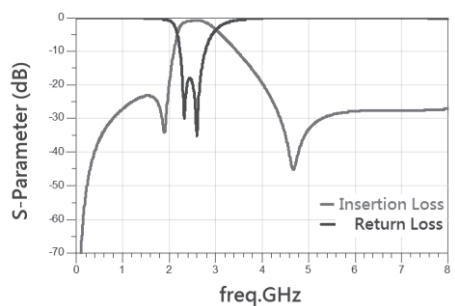
RFBPF1608060ADT
