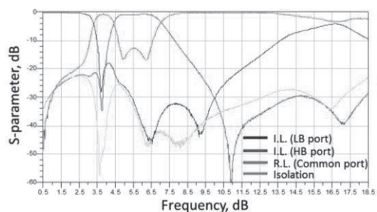
RFDIP2012050L7T
