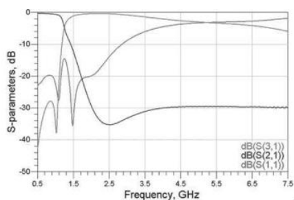
RFDIP2012070G5T
