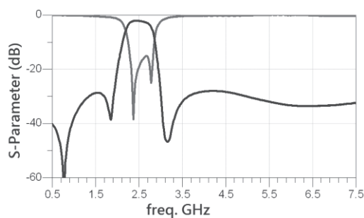
RFBPF1608060A1T
