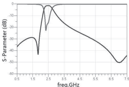
RFBPF1608050A0T
