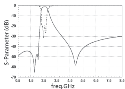
RFBPF2520080AUT
