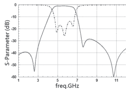
RFBPF1608060K788Q1C
