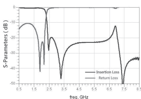
RFLPF1005040A0T
