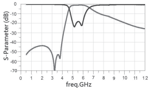
RFBPF2012100K3T
