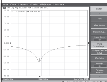
Return Loss (S11)
