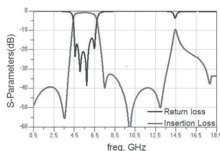
RFBPF1608060K88Q1C
