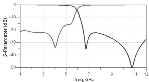
RFLPF3225180Y1T
