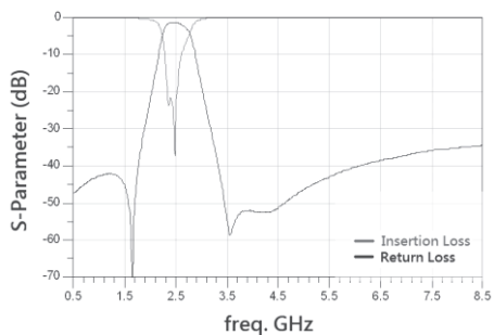
RBBPF1411060A8T
