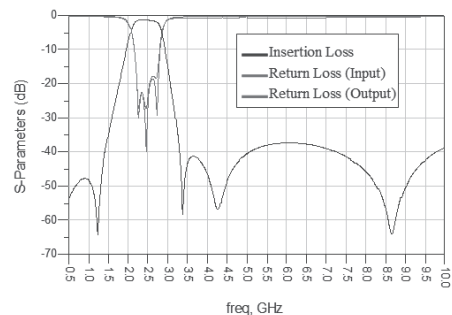
RFBPF2012090A2T
