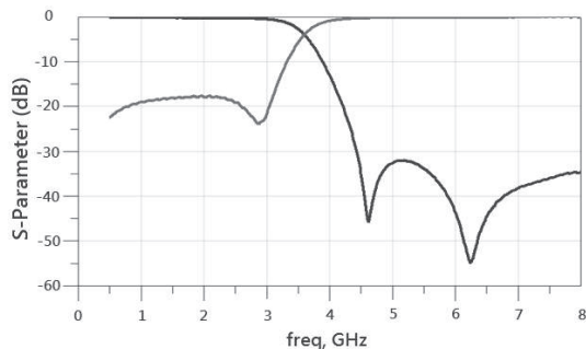
RFLPF16082G5W6T
