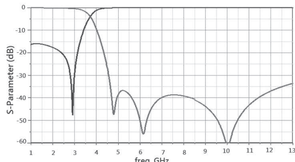
RFLPF16082G5WM0T29
