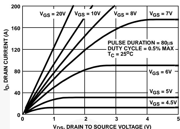
FIGURE 7. SATURATION CHARACTERISTICS
