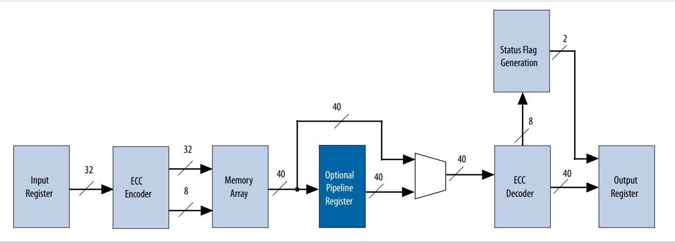
Figure 2-11: ECC Block Diagram for M20K Memory
