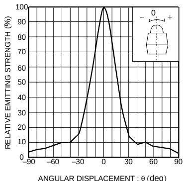
Fig.8 Directional pattern(2)
