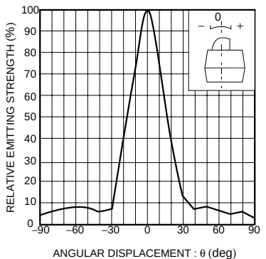
Fig.7 Directional pattern(1)
