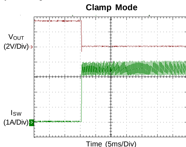
Figure 7. Clamp Mode
