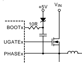
Figure 5. Reducing the UGATEx Rise Time
