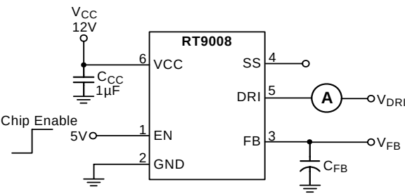
Figure 2. DRI Source/Sink Current Test Circuit
