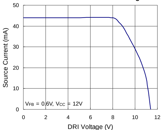
Source Current vs. DRI Voltage
