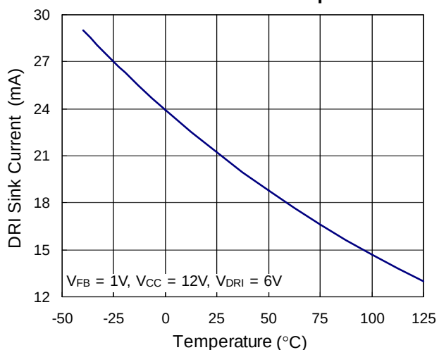
DRI Sink Current vs. Temperature
