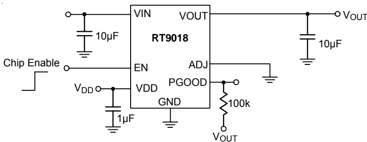
Figure 1. Fixed Voltage Regulator
