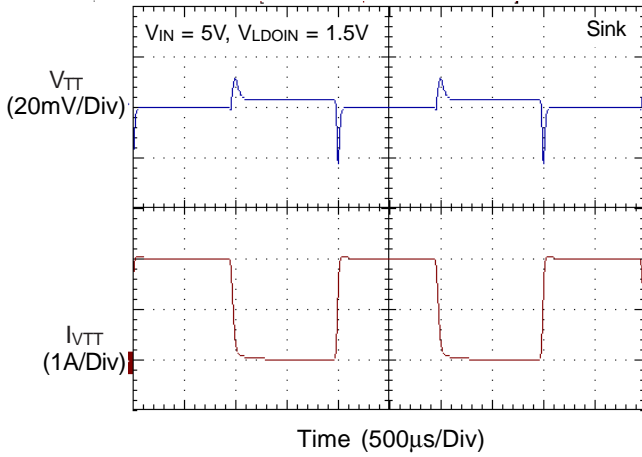
0.75V TT @ 2A Transient Response
