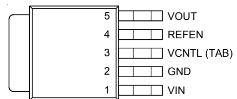
TO-252-5 (RT9173A)
